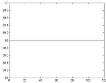
Figure 11. Case 1 plaintext
