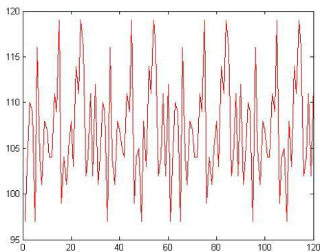
Figure 13. Case 2 plaintext
