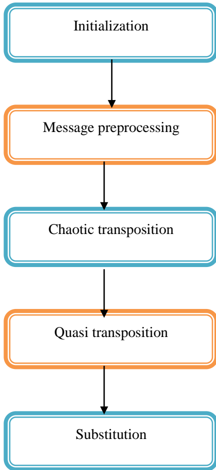
Figure 1(a). Encryption
