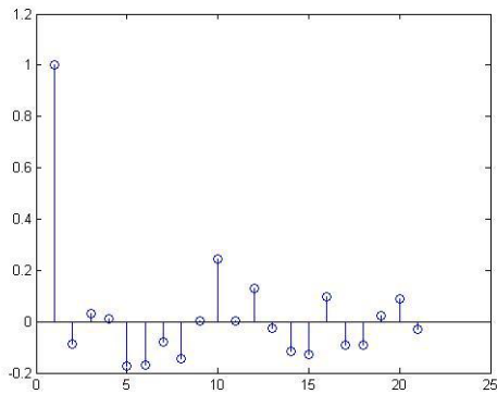
Figure 16. Autocorrelation of case 2 plaintext Figure 17. Autocorrelation of case 2 ciphertext
