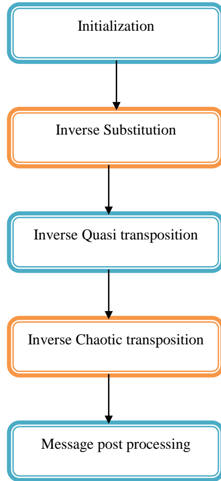
Figure 1(b). Decryption
