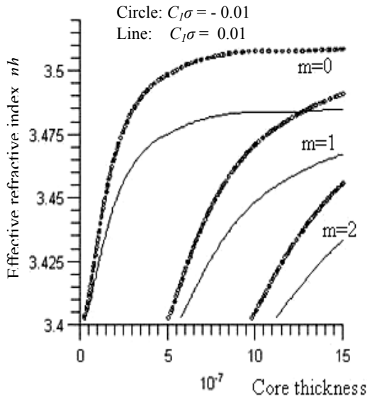
Figure (4): Effective refractive index, n_h , versus the core thickness for the first TM modes in the asymmetric planar optical waveguide under different hydrostatic stresses.
