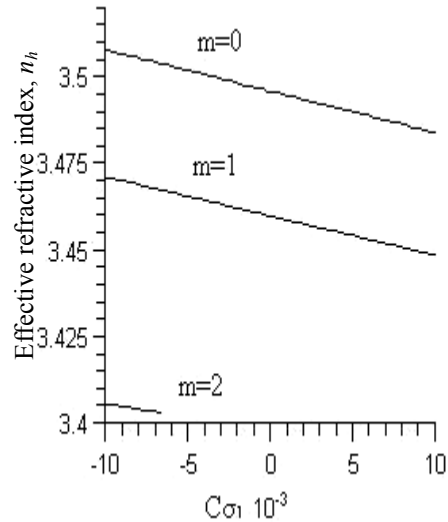
Figure (5): Effective refractive index, n_h , for the first TM modes versus the normalized hydrostatic stress for asymmetric planar optical waveguide with thickness t=1\mu\text{m} .
