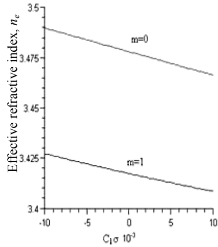
Figure (3): Effective refractive index, n_e , for the first TE modes versus the normalized hydrostatic stress for asymmetric planar optical waveguide with thickness t=1\mu\text{m}
