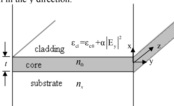
Figure (1): Schematic of asymmetric three layer planer waveguide.
