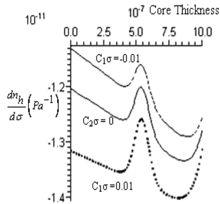
Figure (8): Stress sensitivity of the effective refractive index as a function of core thickness for different stress state for zero mode TM field.
