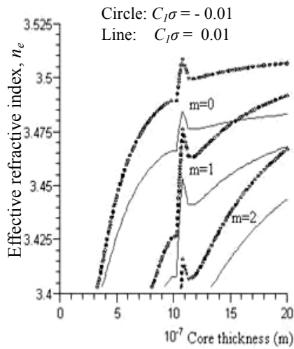
Figure (2): Effective refractive index, n_e , versus the core thickness for the first TE modes in the asymmetric planar optical waveguide under different hydrostatic stresses.
