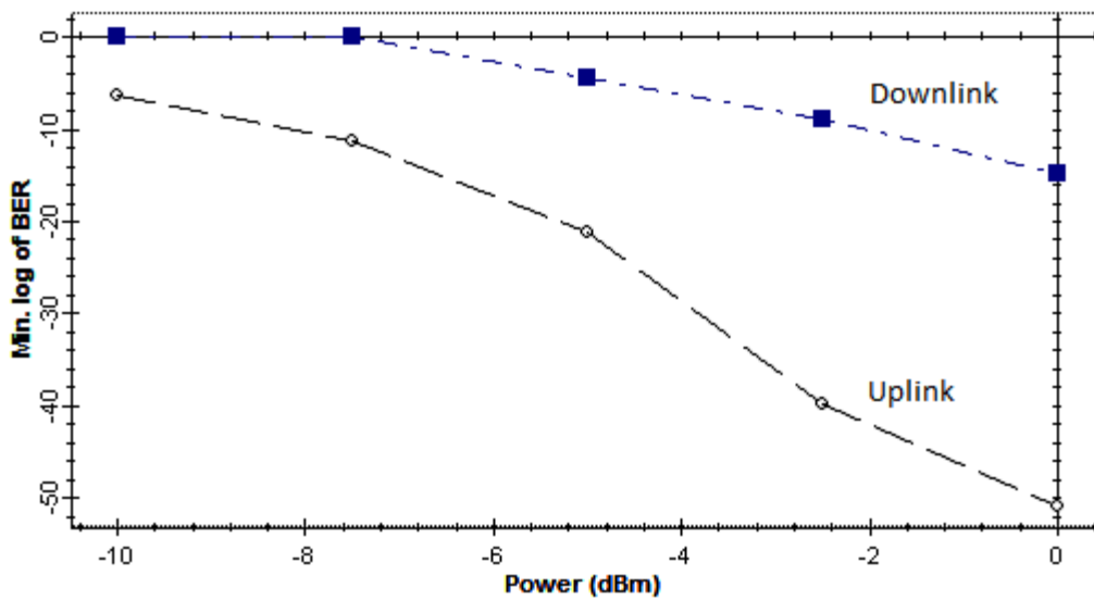
Figure 4: BER versus Input Optical Power
