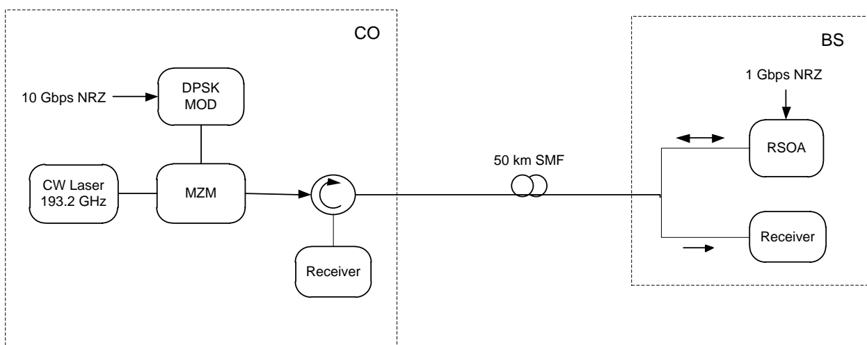
Figure 1: Full-duplex ROF system
