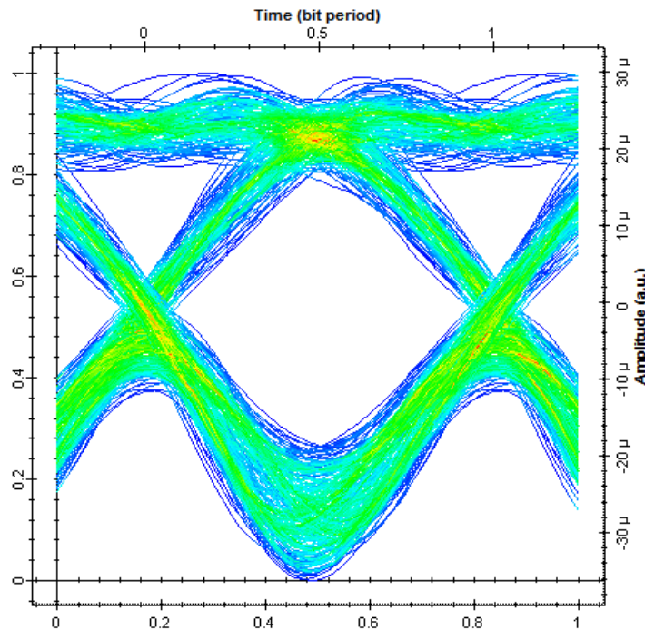
Figure 2: Eye Diagram of de-mod DPSK signal-Downlink
