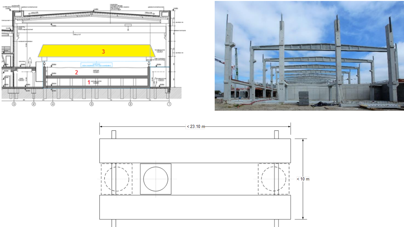
Figure 5 – (top left) Cross section of the towing tank hall showing the water storage (1), test basin (2) and schematic of the carriage (3). (top right) View during construction. (bottom) Carriage top view.
