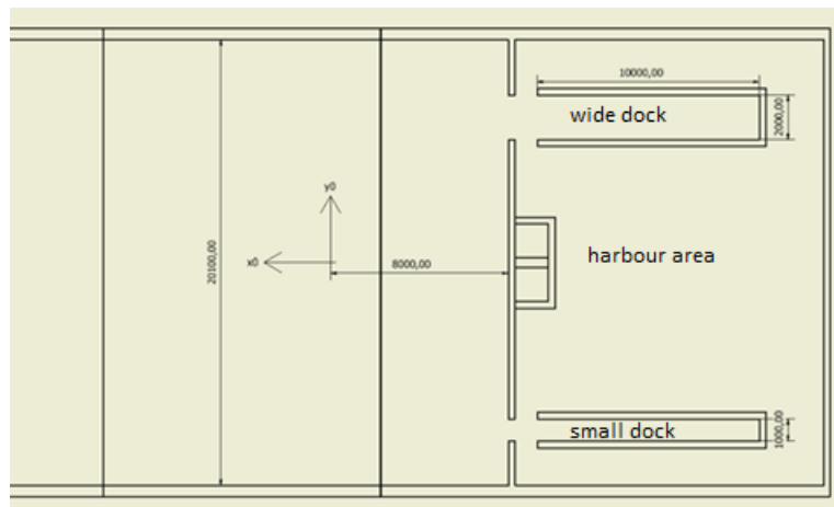
Figure 7– Detail of the tank at the origin of the tank coordinate system. The connections between tank and harbour (with two docks) still needs to be designed hence the opening in between.
