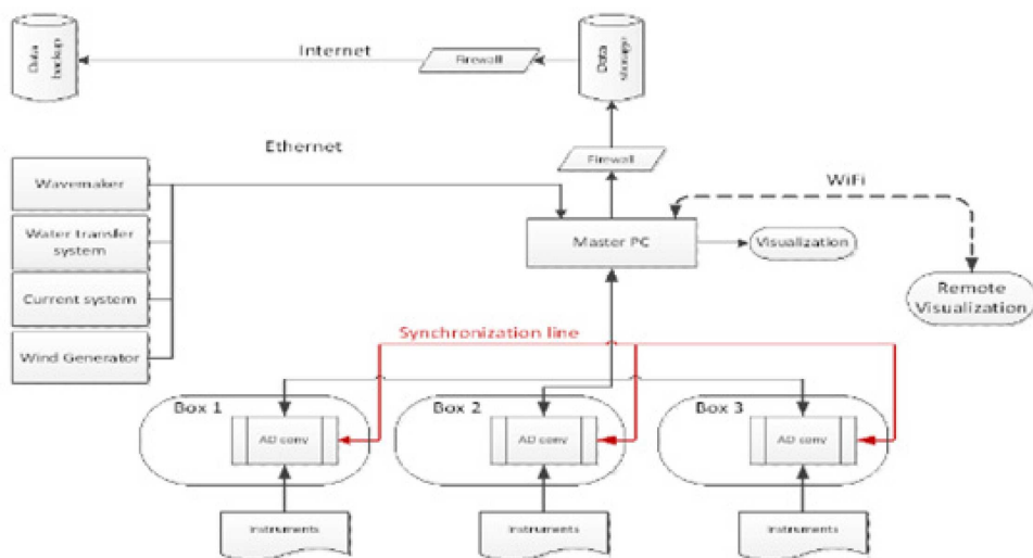
Fig. 5. Schematic of the COB Data Acquisition System
