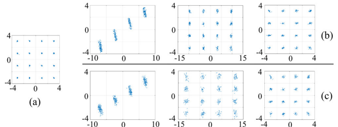
Fig. 5. VPI simulation. (a) 0 km fiber, (b) \alpha_e = 0.5 , 5.5 km fiber and (c) \alpha_e = -0.5 , 8 km fiber. \Phi=90^\circ (left), optimized \Phi to compensate chromatic dispersion (middle), and jointly optimized combiner ratio and \Phi (right).
