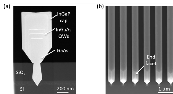
Fig. 1. (a) High-angle annular dark-field scanning transmission electron microscope (HAADF-STEM) image of the cross-section of the GaAs nano-ridge grown on Si substrate considered in this work. (b) Top-view scanning electron microscopy (SEM) images of the nano-ridge array show the irregular shape of the end facets.
