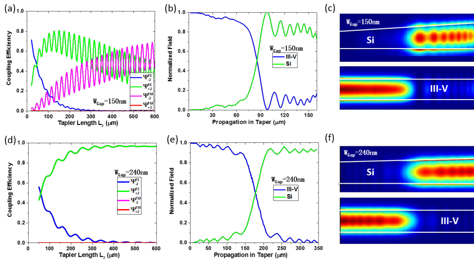
Fig. 7. Simulation results for the configurations (a)–(c) W_{Gap} = 150 nm, W_1 = 235 nm, W_2 = 370 nm, and (d)–(f) W_{Gap} = 240 nm, W_1 = 270 nm, W_2 = 315 nm. (a),(d) show the coupling to several modes as function of taper length L_2 . (b),(e) depict the field exchange between the III-V nano-ridge and Si waveguide along the propagation axis for the optimised taper lengths L_2 = 150 \mu\text{m} and L_2 = 310 \mu\text{m} respectively. (c),(f) Show a 2-D image of the field exchange between the III-V nano-ridge and the Si waveguide for the optimised couplers.
