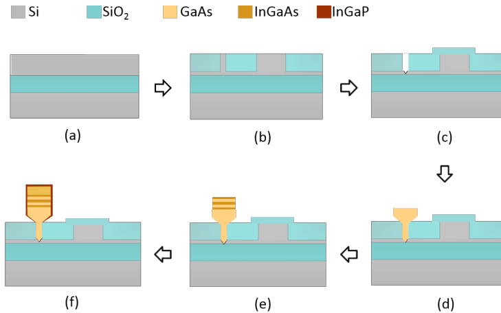
Fig. 3. Proposed process flow of the III-V/Si coupler. (a) The process starts from a SOI wafer. (b) STI process to define high aspect ratio trench and Si WG by lithographic patterning, Si dry etch and SiO 2 deposition and CMP (chemical-mechanical polishing). (c) Prepare SiO 2 trench for III-V epitaxy by Si wet etch. (d) GaAs growth inside and outside the trench. (e) The growth of three InGaAs QWs. (f) A passivation layer of InGaP is deposited to cover the nano-ridge. After this the sample is planarized with SiO 2 , see Fig. 4(a).
