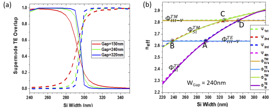
Fig. 6. (a) The overlap between TE-like supermode \Psi_+^{TE} and TE-like modes \Phi_{III-V}^{TE} (solid lines) and \Phi_{Si}^{TE} (dashed lines) of the standalone WGs as a function of W_{Si} for W_{Gap} = 150 nm, 240 nm and 320 nm respectively. (b) The effective refractive indices n_{eff} of the TE/TM-like ground modes of the separated III-V/Si WGs and of the first four supermodes as function of W_{Si} , for W_{Gap} = 240 nm.
