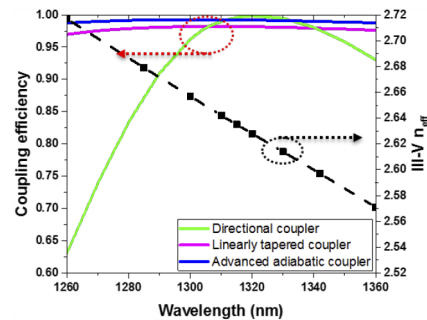
Fig. 10. Coupling efficiency (left axis) and effective refractive index n_{III-V}^{TE} (right axis) as a function of wavelength.
