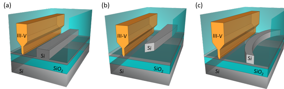
Fig. 2. 3D schematic views of the three coupler implementations. (a) Directional coupler. (b) Linearly tapered coupler. (c) Advanced adiabatic coupler.
