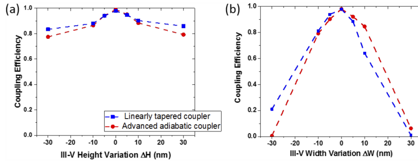
Fig. 11. Coupling efficiency as a function of (a) nano-ridge height variation, (b) width variation.
