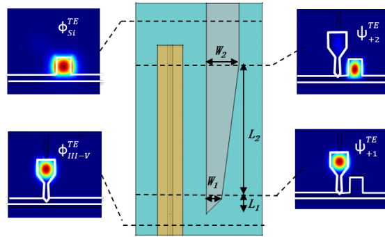
Fig. 5. Top view of the tapered coupler and the field profile of the TE-like modes at different cross-sections of the coupler.
