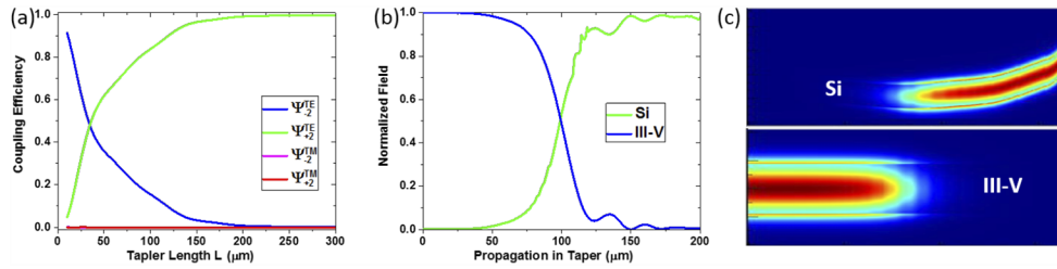
Fig. 9. Simulation results for the optimized adiabatic coupler configuration shown in Fig. 8. (a) The coupling efficiency as a function of coupler length L . A coupling efficiency \eta_C > 99\% can be reached for L = 200 \mu\text{m} . (b) Field exchange between III-V nano-ridge and Si waveguide along propagation direction when W_{Si}(\frac{L}{2}) = W_{\text{match}} = 295 \text{ nm} , W_{Si}(0) = 280 \text{ nm} , W_{Si}(L) = 310 \text{ nm} , W_{\text{Gap}}(\frac{L}{2}) = 150 \text{ nm} , W_{\text{Gap}}(0) = W_{\text{Gap}}(L) = 820 \text{ nm} , L = 200 \mu\text{m} . (c) 2-D image of field exchange between III-V nano-ridge and Si waveguide for L = 200 \mu\text{m} .
