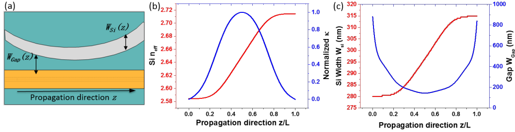
Fig. 8. (a) Top view of the optimized adiabatic coupler. The gap W_{Gap} and Si WG width W_{Si} are functions of the propagation direction z . Note that W_{Gap} is measured from the side of the III-V trench, at the bottom of the nano-ridge, see Fig. 4. (b) The calculated effective refractive index of the Si WG n_{eff} (left axis) and normalized coupling coefficient \frac{\kappa(z)}{\kappa_{max}} as functions of propagation direction z . (c) Calculated Si WG width W_{Si}(z) and gap W_{Gap}(z) along taper.
