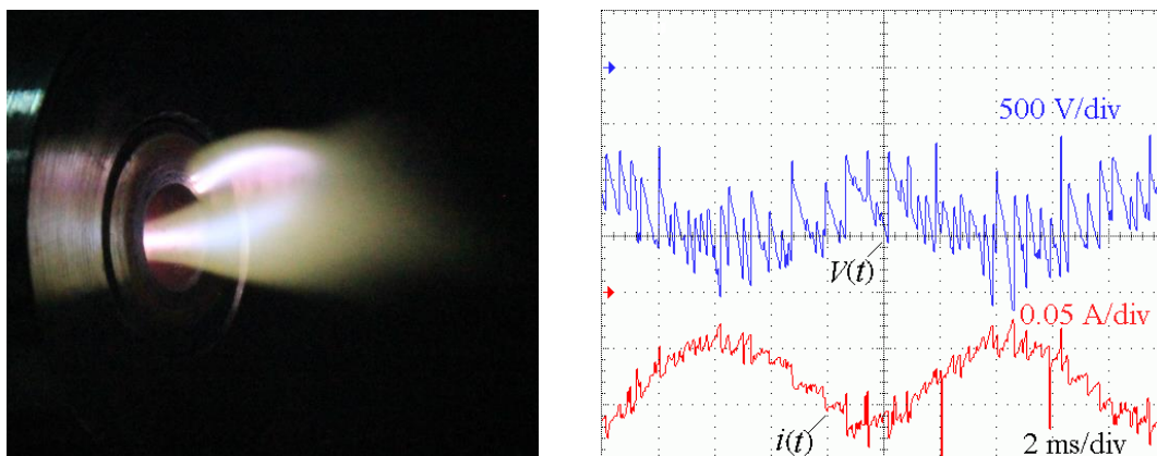
Fig. 1. Photography of plasma jet on the exit of plasmatron nozzle and the glow discharge burning voltage and current waveforms. V(t) – discharge burning voltage, i(t) – discharge current. The gas flow rate G(\text{air}) = 0.1 g/s.
