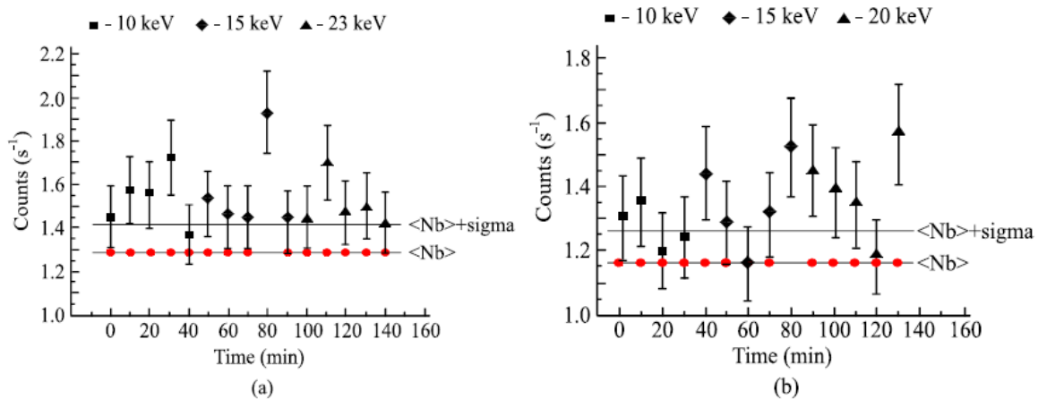
Figure 3. The count of the neutron detector ^3\text{He} (■, ◆, ▲). (a) Target - Ti/TiO 2 :D x 300 \mu\text{m} , beam - H + (10, 15, 23 keV), (b) Target - Ti/TiO 2 :D x 300 \mu\text{m} , beam - Ne + (10, 15, 20 keV). The average background <Nb> (●) is measured with a Cu target.
