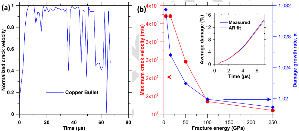
Figure 9. (a) Evolution of normalized crack velocity of a major radial crack in a glass plate with a fracture energy 4.3 \text{ J/m}^2 for a copper bullet. Note that the crack velocity is normalized with respect to the maximum crack velocity during the propagation of the crack. (b) Maximum crack velocity (left axis) and damage growth rate (right axis) with respect to the fracture energy of the glass plate. INSET shows the AR fit compared to the measured evolution of damage in peridynamics simulation of impact on a glass plate with fracture energy 4.3 \text{ J/m}^2 .
