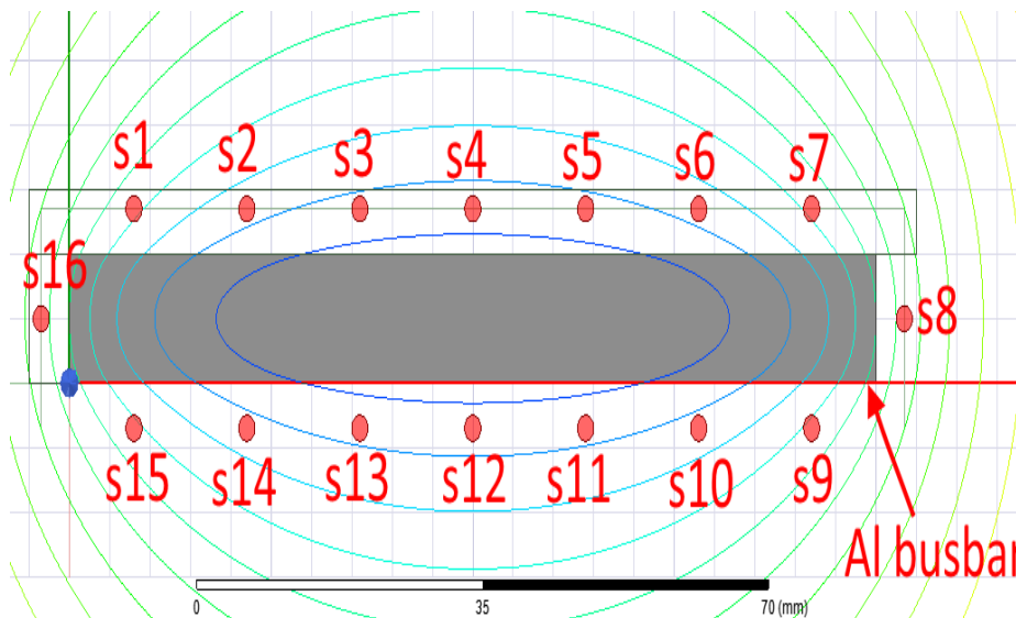
Fig. 5 Rectangular current transducer - location of the sensors [88]
