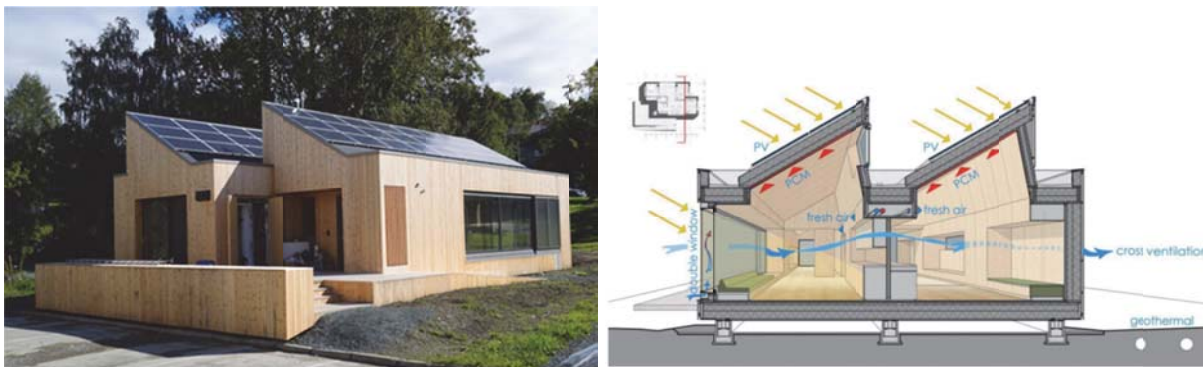
Fig. 1 Photo and Section of the Living Lab (Finocchiaro et al., 2014)
