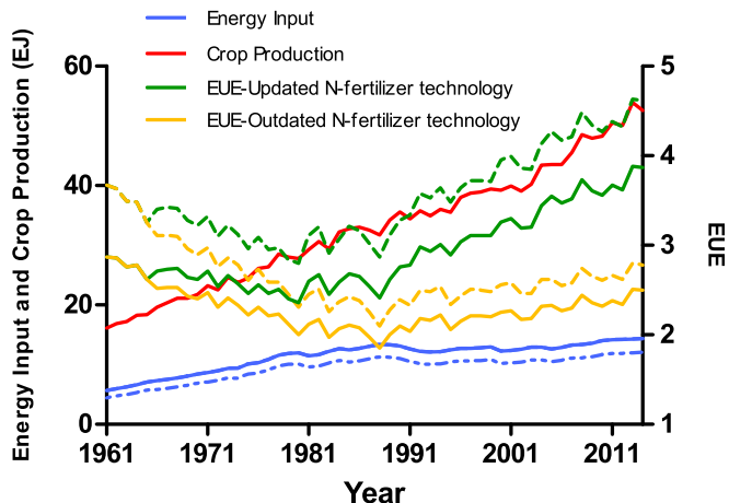
Fig. 2. Total annual energy input (in EJ), crop production (in EJ), and EUE of the 58 main crop-producing countries. “Outdated” and “Updated” N-fertilizer technology refer to industrial energy efficiency in synthesizing ammonia (Supporting Information). Energy input and EUE are presented for two machinery lifespan scenarios: 10 y (solid line) and 30 y (broken line).
