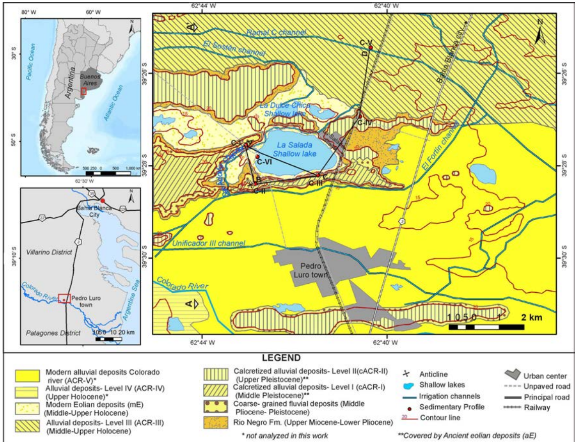
FIG. 2. Geological sketch map (modified after Etcheverría et al. , 2009). The map show the location of the study area, stratigraphic columns and sections analyzed. C-I: Stratigraphic columns I; C-II: Stratigraphic columns II; C-III: Stratigraphic columns III; C-IV: Stratigraphic columns IV; C-V: Stratigraphic columns V; C-VI: Stratigraphic columns VI.
