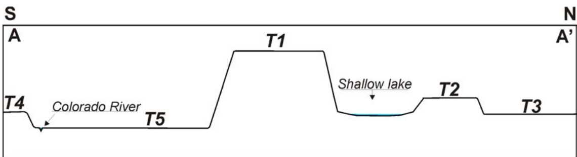
FIG. 3. Schematic cross-section of the line showed as A-A' in the figure 2 representing the topographic relationship of the terraces in the alluvial fan of the Colorado River. These are mentioned as T1, T2, T3, T4, and T5 from oldest to youngest; is not to scale.
