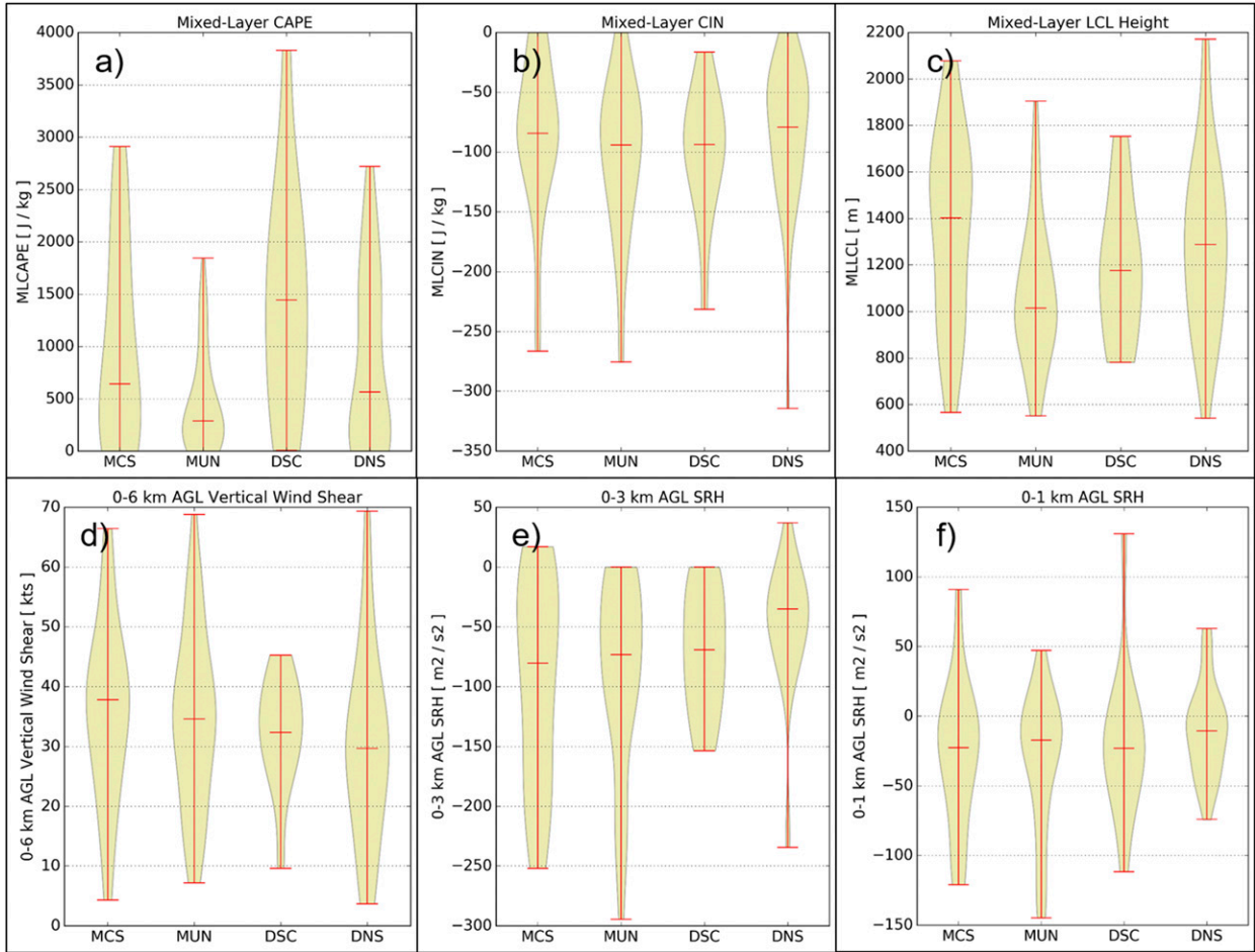
FIG. 16. ERA-Interim composite mean violin boxplots averaged over a 3^\circ \times 3.5^\circ ( 30^\circ – 33^\circ S, 62.5^\circ – 66^\circ W) domain for (a) MLCAPE ( J kg^{-1} ), (b) MLCIN ( J kg^{-1} ), (c) MLLCL height (m), (d) 0–6-km AGL vertical wind shear (kt), (e) 0–3-km AGL SRH ( m^2 s^{-2} ), and (f) 0–1-km AGL SRH ( m^2 s^{-2} ).
