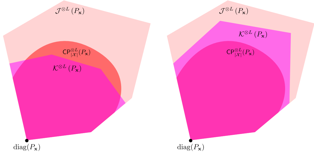
(a) “Below Plotkin point”, positive (L - 1) -list decoding rate is possible. In this case, for some input distribution P_{\mathbf{x}} \in \lambda_{\mathbf{x}} , the slice of P_{\mathbf{x}} -self-coupling CP tensors is not entirely contained in the confusability set \mathcal{K}^{\otimes L}(P_{\mathbf{x}}) .
