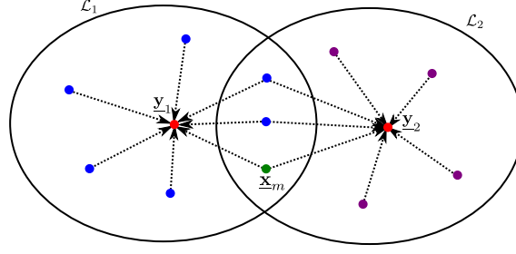
■ Figure 5 \mathcal{E} \subset \mathcal{E}_1 \cap \mathcal{E}_2 \cap \mathcal{E}_3 . We upper bound \Pr[\mathcal{E}] by neglecting the fact that codewords \underline{x}_i for i \in (\mathcal{L}_1 \cap \mathcal{L}_2) \setminus \{m\} are simultaneously \underline{y}_1 -confusable and \underline{y}_2 -confusable, or equivalently, neglecting that \underline{y}_1, \underline{y}_2 should simultaneously belong to \mathcal{A}_{\underline{y}|\underline{x}_{m'}} for all m' \in \mathcal{L}_1 \cap \mathcal{L}_2 , not only the particular m we have chosen.
