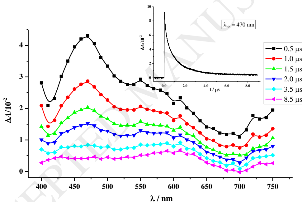
Figure 9: Transient spectra recorded at different delays after the laser pulse in flash photolysis experiments of P4VP-Re(dppz) in deaerated DMF. Inset show an oscillographic trace at \lambda_{\text{ob}} = 470 . See text for details.
