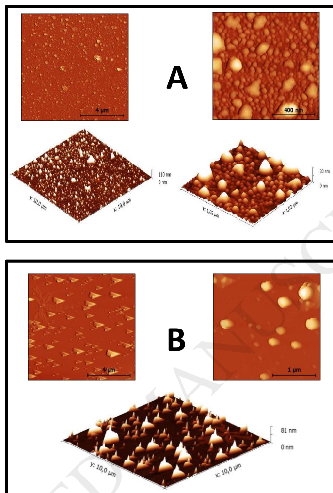
Figure 5: AFM images for P4VP-Re(dppz) in DMF (top panel A ) and DMF/HClO 4 0.05 M (bottom panel B )
