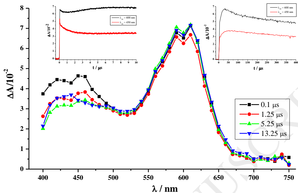
Figure 11: Transient spectra recorded at different delays after the laser pulse in flash photolysis experiments of P4VP-Re(dppz) in deaerated DFM containing TEOA 0.075 M. Insets show oscillographic traces at \lambda_{\text{ob}} = 450 and 600 nm in the 0-10 \mu\text{s} time range (left panel) and in the 0-400 \mu\text{s} time range (right panel). See text for details.
