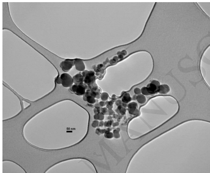
Figure 3. TEM images of P4VP-Re(dppz) polymer films prepared with [\text{Re(I)}] = 2 \times 10^{-5} M in DCM. See text for details.
