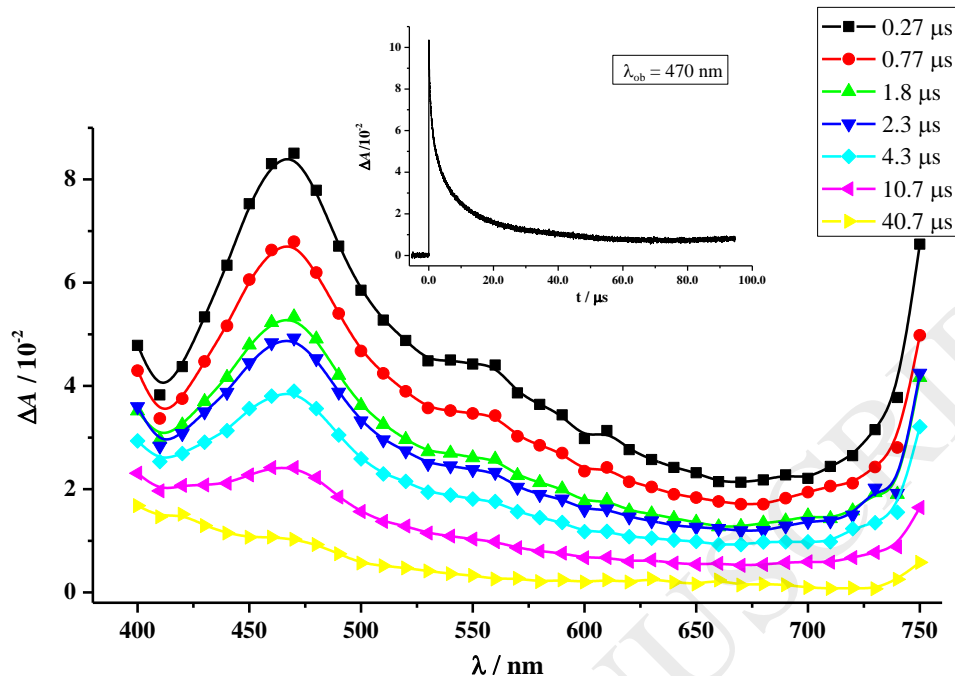
Figure 10: Transient spectra recorded at different delays after the laser pulse in flash photolysis experiments of P4VP-Re(dppz) in deaerated DFM/HClO 4 0.05 M. Inset show an oscillographic trace at \lambda_{\text{ob}} = 470 . See text for details.
