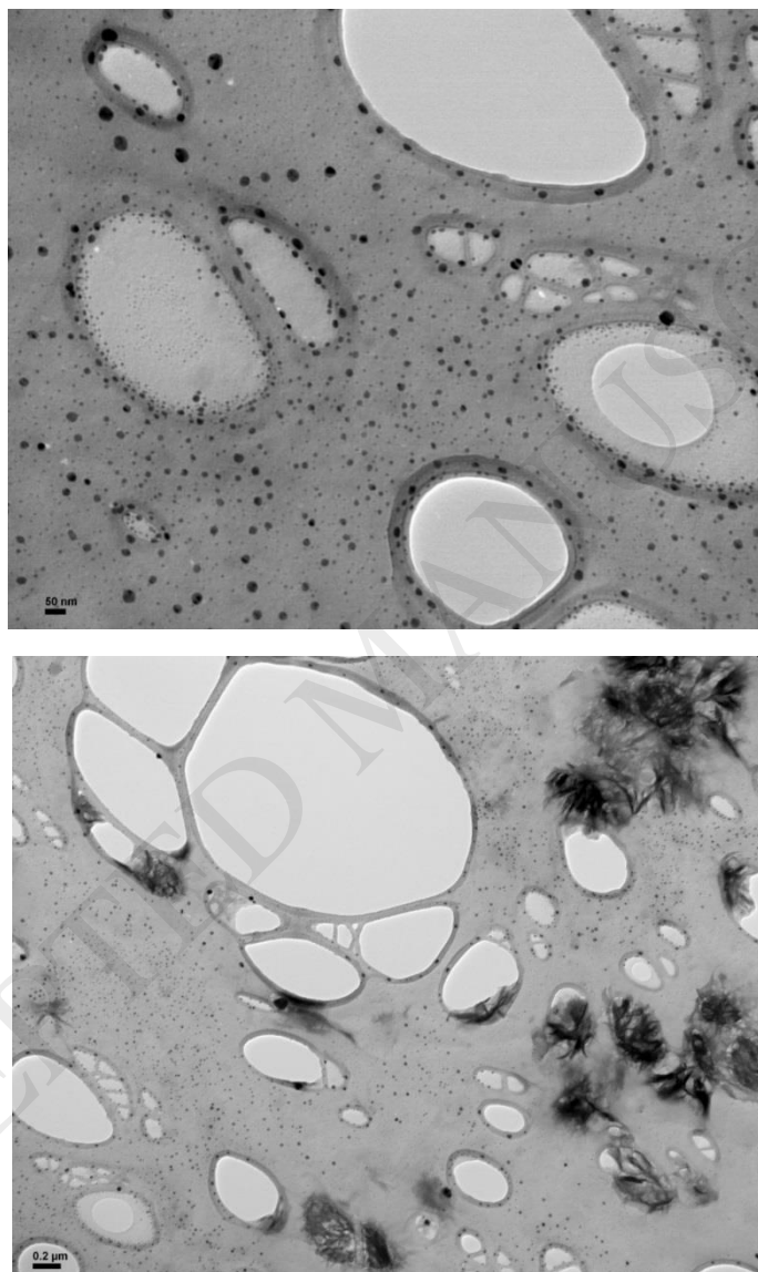
Figure 2. TEM images of P4VP-Re(dppz) polymer films prepared with [\text{Re(I)}] = 2 \times 10^{-5} M in DMF/HClO 4 . See text for details
