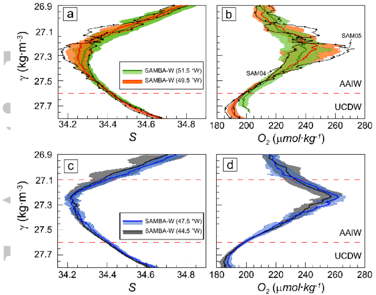
Figure 11. Same as Fig. 10 for the intermediate layer. Two individual CTD profiles collected at 49.5 °W during SAM04 (December 2010) and SAM05 (July 2011) cruises are shown in black in (a) and (b).
