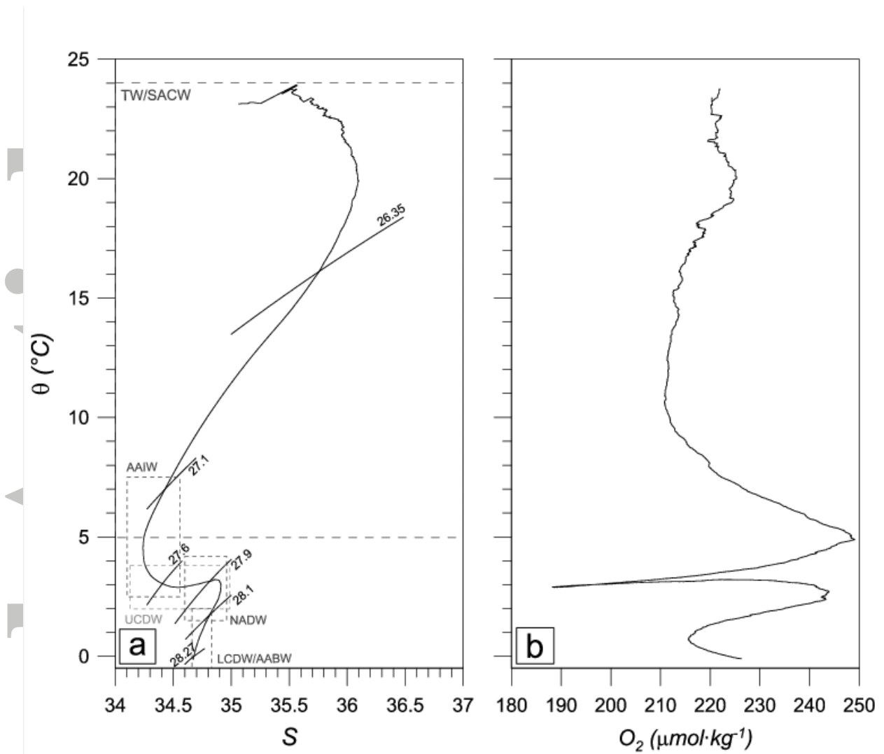
Figure 4. Zonally averaged, time-mean (a) \theta - S and (b) \theta - O_2 distribution along the SAMBA-W line using all CTD profiles collected within the SAMOC initiative and all available Argo profiles in the region (see Fig.1 for location). The dashed boxes in (a) indicate the domains of the water masses discussed in Figs. 5 to 9. The solid lines are the \sigma_t surfaces used to delimit the water masses (see text for details on the determination of these).
