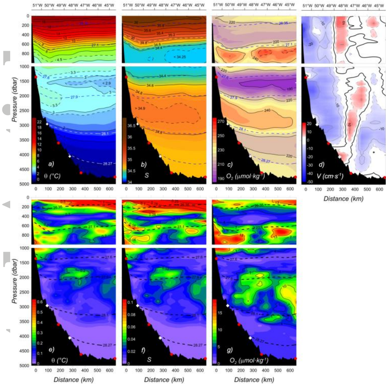
Figure 3. (a-c) Average sections of potential temperature ( \theta ), salinity ( S ) and dissolved oxygen concentration ( O_2 ) at the SAMBA-W line using all CTD profiles collected within the SAMOC initiative and all available Argo profiles in the region (see Fig.1 for CTD and Argo profiles locations). (d) Average section of the alongshore velocity ( V ) derived from LADCP measurements. (e-f) Standard deviation sections of \theta , S and O_2 at the SAMBA-W line using only CTD profiles collected within the SAMOC initiative. The red circles (white diamonds) in all panels indicate the PIES (CPIES) locations. The dashed lines indicate the averaged \gamma surfaces used to delimit the water masses. Note that the section changes orientation west of the x -axis origin (Fig. 1c).
