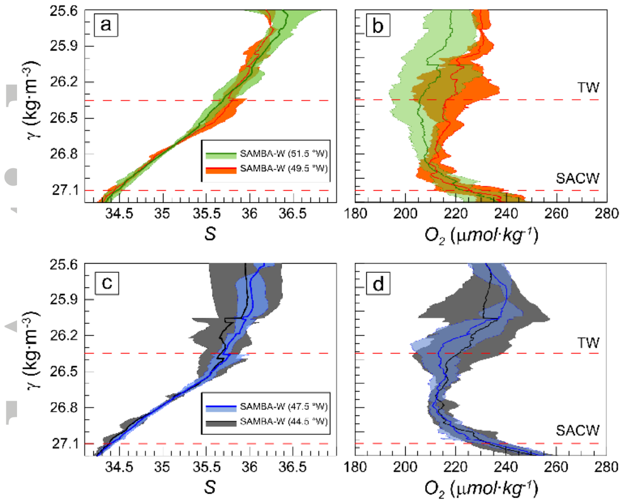
Figure 10. Time-mean profiles of (a,c) S and (b,d) O_2 computed along neutral density ( \gamma ) surfaces for the upper layer at four selected longitudes along the SAMBA-W line. The shading in all panels indicates the standard deviation for each density level. The red dashed lines are the \gamma surfaces used to delimit each water mass. The water mass layers are indicated in (b) and (d).
