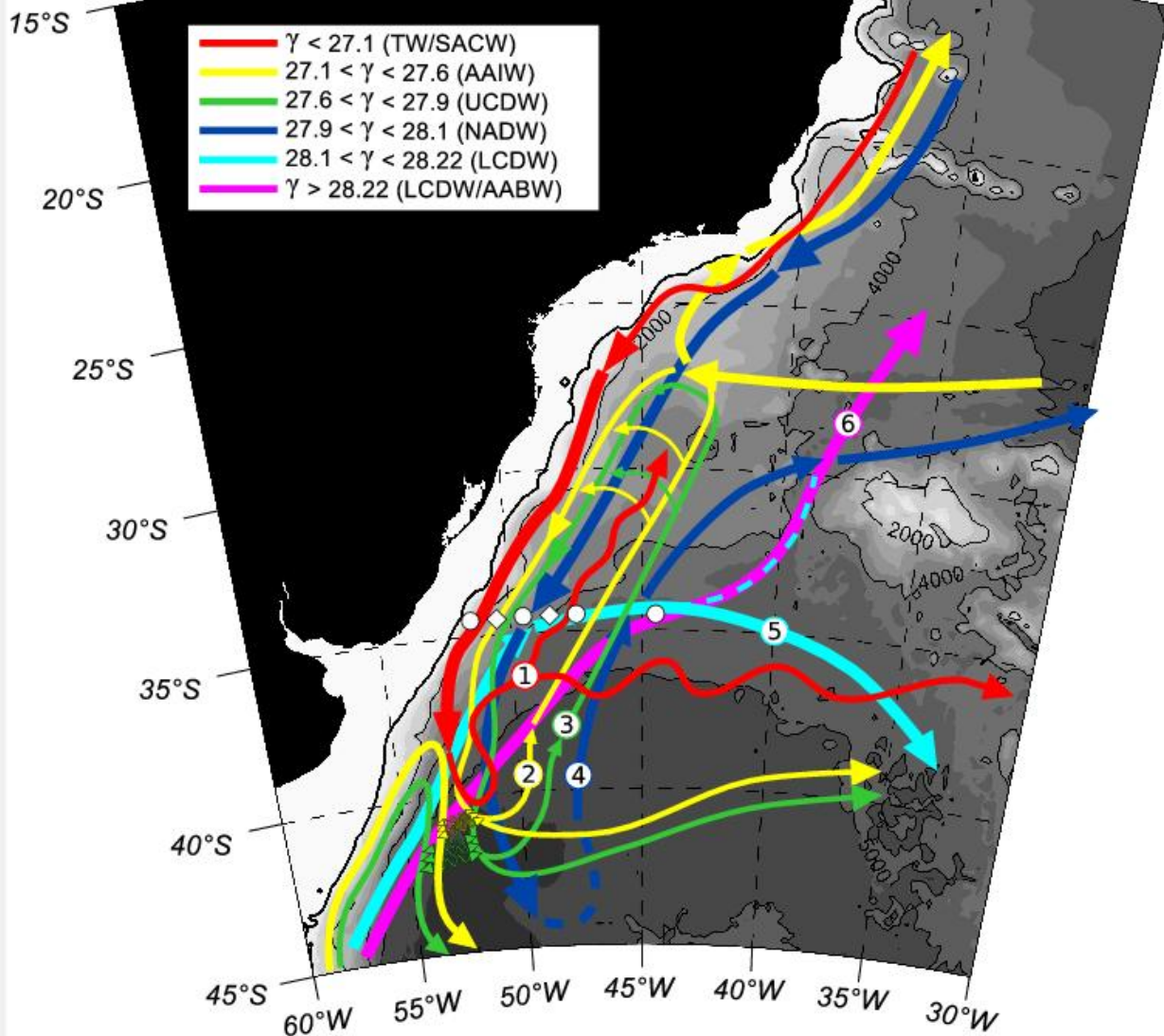
Figure 13. Schematic pathways of the water masses in the northwest Argentine Basin, colored coded according to the different layers defined by neutral density ranges (in \text{kg}\cdot\text{m}^{-3} ) as indicated. The water masses associated to each density range are also indicated. The main pathways are numbered for reference in Section 5. The zigzag yellow and green arrows indicate property exchanges in the BMC region and the dashed paths indicate sporadic or unconfirmed pathways. The white circles (diamonds) indicate the PIES (CPIES) locations along the SAMBA-W line for reference. The bathymetry has been taken from Fig. 1.
