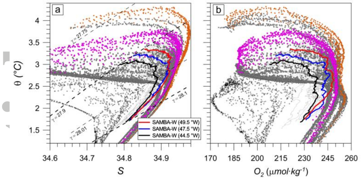
Figure 8. Same as Fig. 5 for the NADW layer. The orange (grey) diamonds are CTD profiles collected within (farther than) 300 km of the 200 m isobath at the CITHER-2 LEG 2 section (13 °S); the magenta (grey) circles are CTD profiles collected within (farther than) 200 km of the 200 m isobath at the CLIVAR/WOCE A10 (~ 30 °S); the black crosses are CTD profiles collected during the CITHER-2 LEG 1 (WOCE A17, 45-48 °S) section. The CTD data collected at the SAMBA-W line are bounded to the NADW \gamma limits, all other data are limited to \gamma > 27.7 \text{ kg}\cdot\text{m}^{-3} . See Fig. 1 for CTD stations locations.
