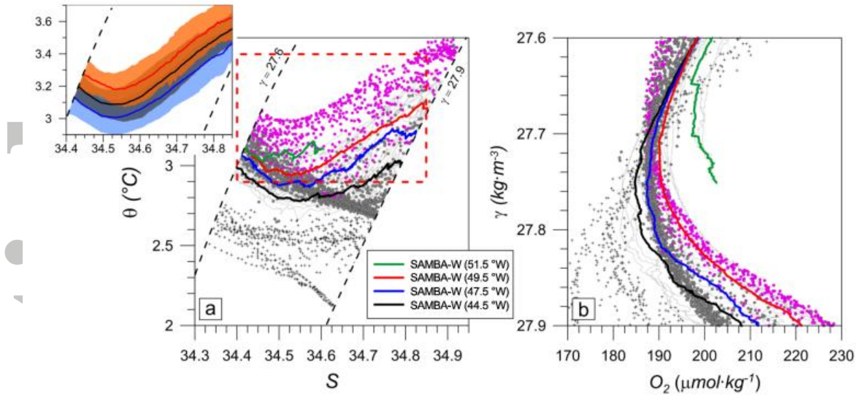
Figure 7. Same as Fig. 5 for the UCDW layer, except (b) is a \gamma vs. O_2 distribution. The magenta (grey) circles in both panels are CTD profiles collected within (farther than) 500 km of the 200 m isobath at the CLIVAR/WOCE A10 sections ( \sim 30 ^{\circ}\text{S} ) and the black crosses are CTD profiles collected at the CITHER-2 LEG 1 (WOCE A17, 45–48 ^{\circ}\text{S} ) section. The inset in (a) shows the \theta - S distribution along the western boundary from Argo data at three selected latitude ranges: 34-31.5 ^{\circ}\text{S} (blue), 31.5-29 ^{\circ}\text{S} (black) and 29-27.5 ^{\circ}\text{S} (red). The heavy lines (shading) are the profile averages (standard deviation). The red dashed rectangle in (a) indicates boundaries of the inset. See Fig. 1 for CTD stations and Argo profiles location.
