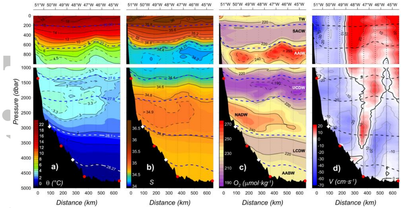
Figure 2. Synoptic sections of (a) potential temperature ( \theta ), (b) salinity ( S ), (c) dissolved oxygen concentration ( O_2 ) and (d) alongshore velocity ( V ) at the SAMBA-W line collected during SAM-07 cruise in July 2012. The red circles (white diamonds) in all panels indicate the PIES (CPIES) locations and the vertical dotted lines indicate the location of the CTD/LADCP stations. The blue and white dashed lines indicate the \gamma surfaces used to delimit the water masses. Note that the section changes orientation west of the x -axis origin (Fig. 1c). The water masses are indicated in (c).
