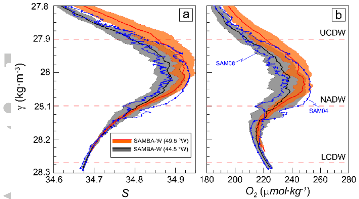
Figure 12. Same as Fig. 10 for the deep and abyssal layers, except only the profiles at 49.5 °W and 44.5 °W are shown. Two individual CTD profiles collected at 44.5 °W during SAM04 (December 2010) and SAM08 (December 2012) cruises are shown in blue.
