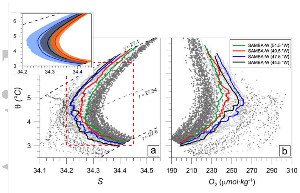
Figure 6. Same as Fig. 5 for the AAIW layer. The grey circles and black crosses in both panels are CTD profiles collected during the CLIVAR/WOCE A10 (~ 30 °S) and CITHER-2 LEG 1 (WOCE A17, 45-48 °S) sections, respectively. The inset in (a) shows the \theta - S distribution along the western boundary from Argo data at three selected latitude ranges: 34-31.5 °S (blue), 31.5-29 °S (black) and 29-27.5 °S (red). The heavy lines (shading) are the profile averages (standard deviation). The red dashed rectangle in (a) indicates boundaries of the inset. See Fig. 1 for CTD stations and Argo profiles location.
