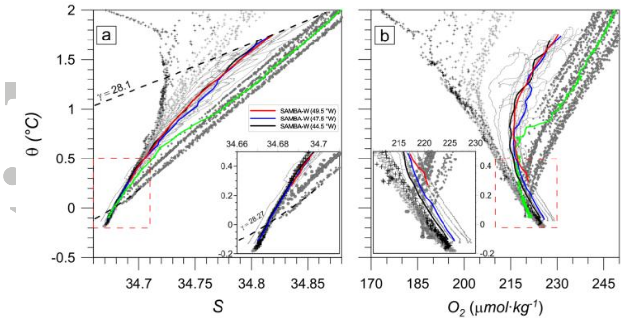
Figure 9. Same as Fig. 5 for the LCDW/AABW layer. The black (grey) crosses in both panels are CTD profiles collected within (farther than) 200 km of the 200 m isobath at the CITHER-2 LEG 1 (WOCE A17, 45-48 °S) section. The circles and diamonds are CTD stations occupied at the CLIVAR/WOCE A10 (~ 30 °S) and the CITHER-2 LEG 2 (13 °S) sections, respectively. The green curve is an individual CTD station collected during the 2011 WOCE A10 section at the Vema Channel near 39.4 °W, 30 °S. The bottom layer is expanded in the insets. See Fig. 1 for CTD stations locations.
