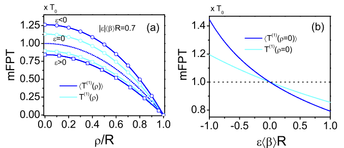
FIG. 1: Mean first passage time (mFPT) \langle T^{(1)}(\rho) \rangle in presence of a constant uncorrelated radial force in 3D [Eq. (15)] and Gamma distributed \beta -fluctuations [Eq. (17)]. T^{(1)}(\rho) is the solution in absence of fluctuations, p(\beta) = \delta(\beta - \langle \beta \rangle) . Time is measured in units T_0 = \langle \beta \rangle R^2/6 . (a) Dependence on the initial position \rho , for negative (circles), null (dotted line), and positive (squares) forces. The parameters fulfill |\varepsilon| \langle \beta \rangle R = 0.7 . (b) Dependence with the external dimensionless force \varepsilon \langle \beta \rangle R at the initial position \rho = 0 .
