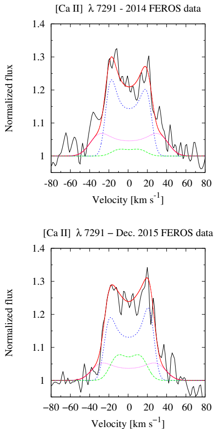
Fig. 20. Model fits to the [Ca II] \lambda 7291 profiles corresponding to the FEROS spectra (2014 and Dec 2015 data, top and bottom panels, respectively). The computed profiles (in red line) were obtained combining different emission structures with different projected Keplerian rotational velocities (see Table 1). The [Ca II] \lambda 7291 line from Nov 2015 FEROS data could not be modelled since it is very noisy.
