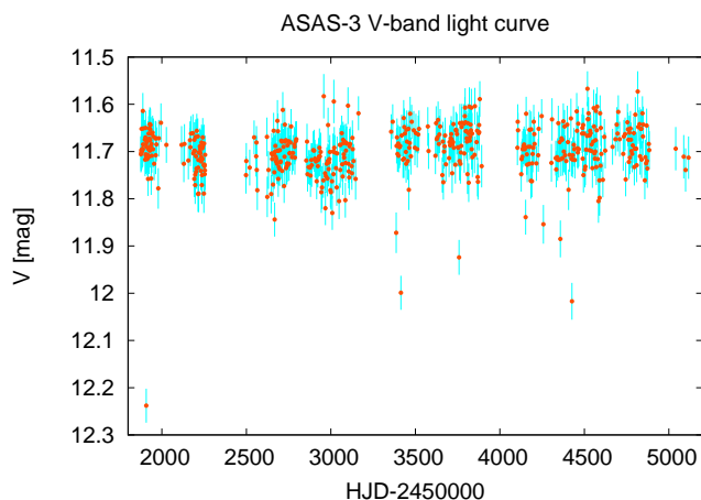
Fig. 21. ASAS-3 V-band light curve of LHA 120-S 35. Although no reliable period was found to describe the variations, a sort of long period ( P > 1750 d) oscillation may be present on which there may be overlapping irregular light variations with amplitudes of about 0.2 mag.
