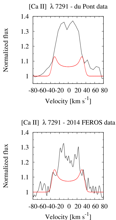
Fig. 16. Comparison between the observed [Ca II] \lambda 7291 line profile from the du Pont and 2014 FEROS spectra (top and bottom panels, respectively) and a computed theoretical profile considering a single ring model. Assuming the same rotational velocity as for the CO ring ( V_{\text{rot}} = 35 \text{ km s}^{-1} ), the broadest part of the [Ca II] \lambda 7291 line profile could be reproduced (data shown in black line, and the model in red).
