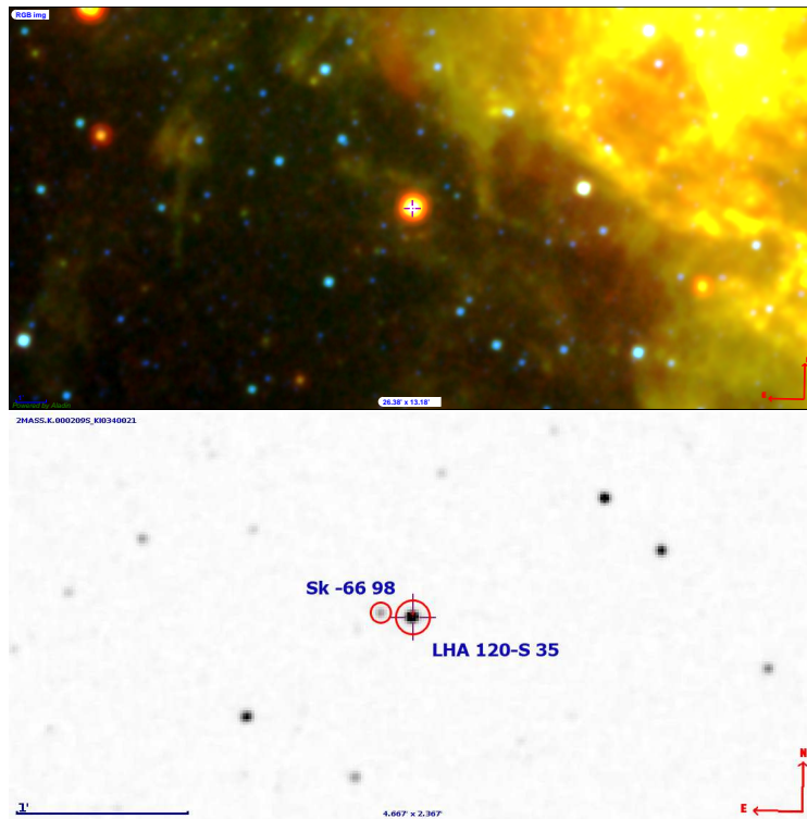
Fig. 22. Top panel: Representative colour RGB WISE image ( \sim 26 \times 13 arcmin 2 ) of LHA 120-S 35 and its surroundings made from images at 4.6 \mu\text{m} (in blue), 12 \mu\text{m} (in green) and 22 \mu\text{m} (in red) with an angular resolution of 6.4, 6.5 and 12.0 arcsec, respectively. Bottom panel: 2MASS K -band image ( \sim 4.7 \times 2.4 arcmin 2 ) showing LHA 120-S 35 (indicated by a cross) along with the neighbouring star Sk -66 98, which remains unresolved in the WISE image. Both images are orientated north up and east to the left.
