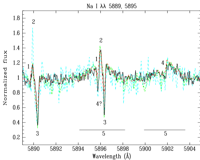
Fig. 8. Na I lines at \lambda\lambda 5889, 5895 Å of LHA 120-S 35 seen in the du Pont and FEROS spectra. The doublet has different velocity components related to different formation regions (see text for more details about the labels).
