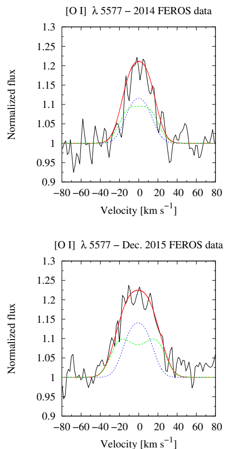
Fig. 18. Model fits to the [O I] \lambda 5577 line profiles corresponding to the FEROS data (2014 and Dec 2015 data, top and bottom panels, respectively). The [O I] \lambda 5577 line from Nov 2015 FEROS spectra could not be modelled since it is very noisy.
