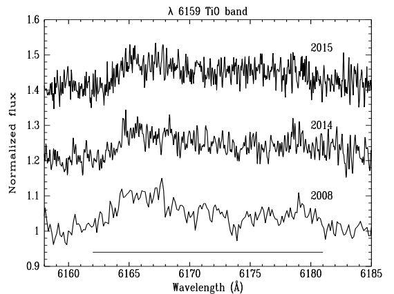
Fig. 12. Detection of a weak TiO band emission in the high-resolution optical spectra of LHA 120-S 35. The TiO feature from the Nov 2015 data is not included since it is very noisy.
