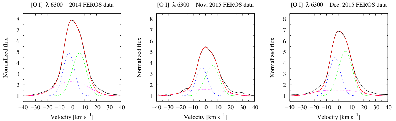
Fig. 19. Model fits to the [O I] \lambda 6300 line profiles corresponding to the FEROS spectra (2014, Nov 2015 and Dec 2015 data, left, middle and right panels, respectively). The computed profiles (in red line) were obtained combining different emission structures with different projected Keplerian rotational velocities (see Table 1).
