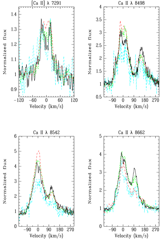
Fig. 11. Comparison of the strength and shape of the [Ca II] \lambda 7291 and the Ca II \lambda 8498, 8542, 8662 emission lines seen in the du Pont data and in FEROS spectra from 2014 and 2015. The Ca II triplet lines are blended with the Paschen lines Pa16, Pa15 and Pa13, respectively.
