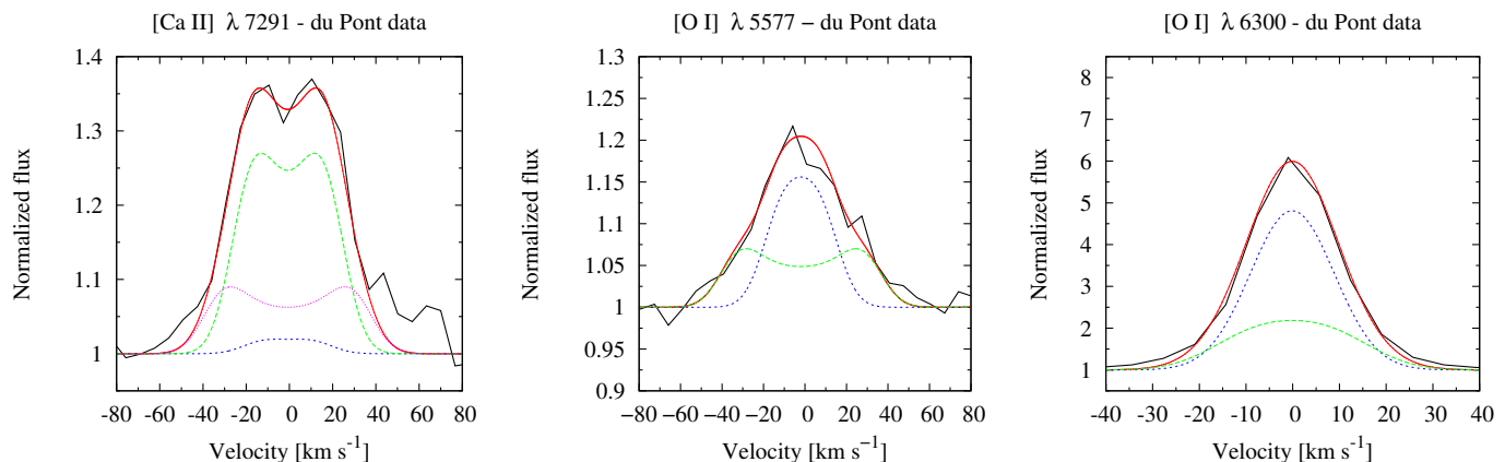
Fig. 17. Model fits to the [Ca II] \lambda 7291 (left panel), [O I] \lambda 5577 (middle panel) and [O I] \lambda 6300 (right panel) line profiles corresponding to the du Pont data. The computed profiles (in red lines) were obtained combining different emitting rings (in other colours) with different projected Keplerian rotational velocities (see Table 1).
