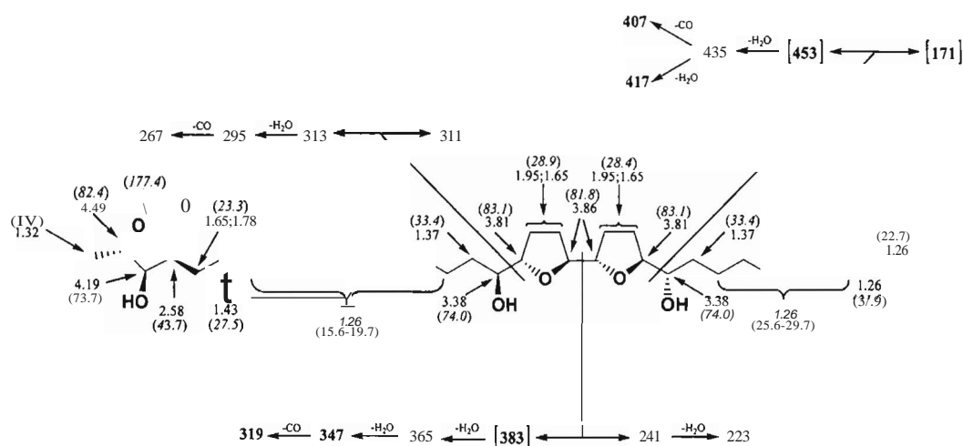
Fig. 1 ^1H - ^{13}C NMR heteronuclear correlations ( ^{13}C in parentheses) spectral data, and significant EIMS fragment ions of tuconanin (1).
