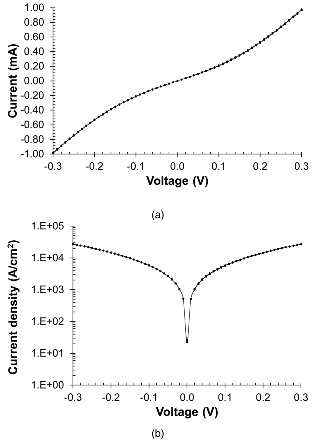
Fig. 5. (a) Measured I - V dependence. (b) Current density (in \text{A}/\text{cm}^2 ) of the MIM diode in the \pm 300 mV voltage range.
