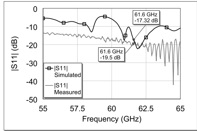
Fig. 8. Comparison between measured and simulated return loss |S_{11}| of the rectenna.
