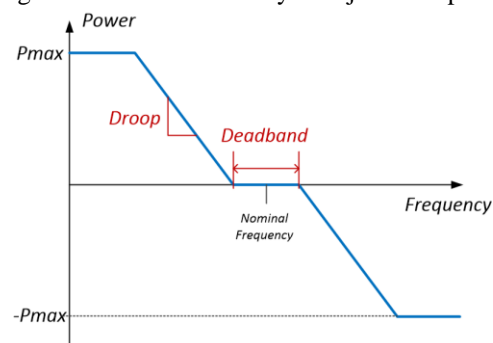
Fig. 1. Droop based frequency response
