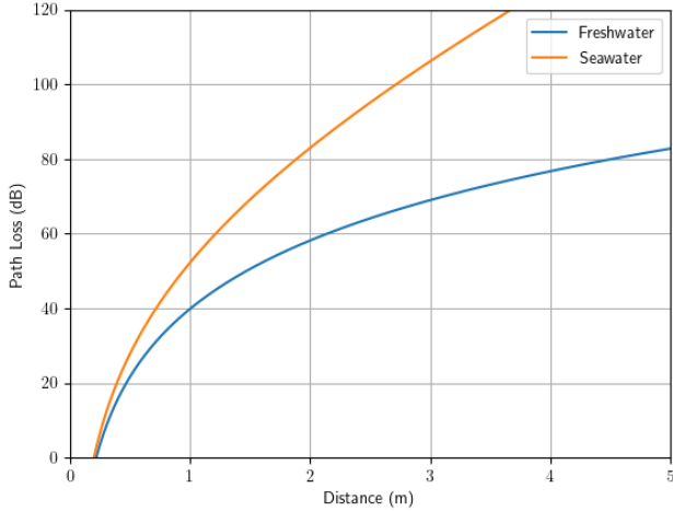
Figure 4. Path loss for an inductively coupled system operating at f = 134.2\text{kHz} .
