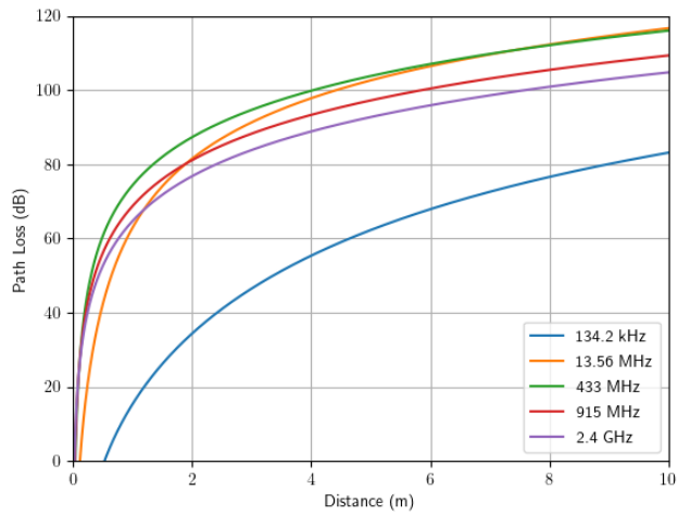
Figure 9. Path loss for RF as a function of distance for two dipole antennas in seawater using \alpha l .
