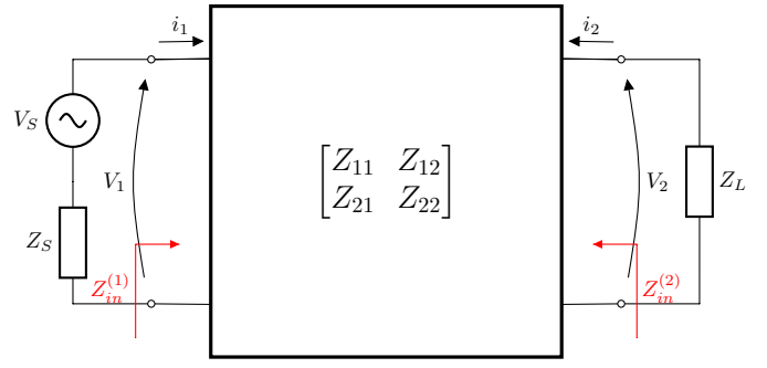
Figure 3. Two-port network equivalent of the system.
