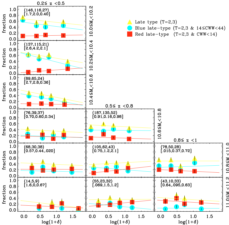
Fig. 12. Contribution of the various spectrophotometric types to the late-type population in different environments. The percentage of the whole morphologically classified late-type population, as well as the percentage of the spectral type subclasses, is plotted as a function of the mass-weighted galaxy overdensity computed using the 5th nearest neighbour density estimator with volume-limited tracers. The redshift increases from the left to the right (as indicated on the top) while objects are progressively more massive from top to bottom (as indicated on the right). The entire late-type population is represented with filled yellow triangles. This population is then divided into 2 subclasses according to the galaxy spectral type: filled cyan circles represent early and late spirals fitted by the templates 14–43; red late-types ( CWW \leq 13 ) are represented with red filled squares. Irregular and starburst spectral types ( CWW > 43 ) are not shown, since they are not present at the masses considered. Enclosed in parenthesis are the total number of objects in the mass and redshift bin considered, as well as the number of blue and red late-type objects. Within square brackets we give the significance of the deviation from zero of the slope of the linear fit.
