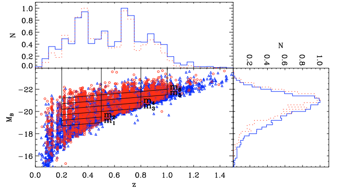
Fig. 1. Central panel: the relation between absolute B -band magnitudes and redshifts is shown as a function of the galaxy morphological type for the 10 k zCOSMOS “bright” galaxy catalogue. Red empty dots represent early-type and blue empty triangles late-type galaxies. The black boxes identify the limits for the subsample selection. Top panel: normalised distribution of early (red dotted line) and late-type (blue solid line) galaxies as a function of redshift. Right panel: normalised distribution of early (red dotted line) and late-type (blue solid line) galaxies as a function of M_B absolute magnitude.
