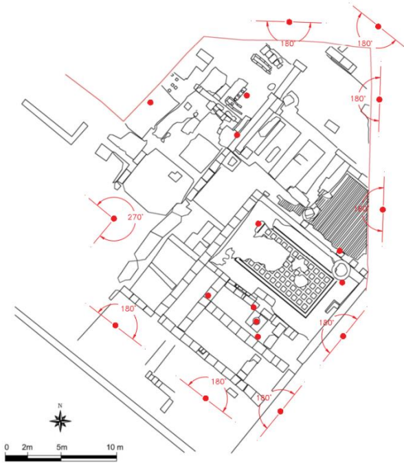
Figure 7: TLS survey of the Sanctuary of Isis area with the positioning of external and internal scans.
