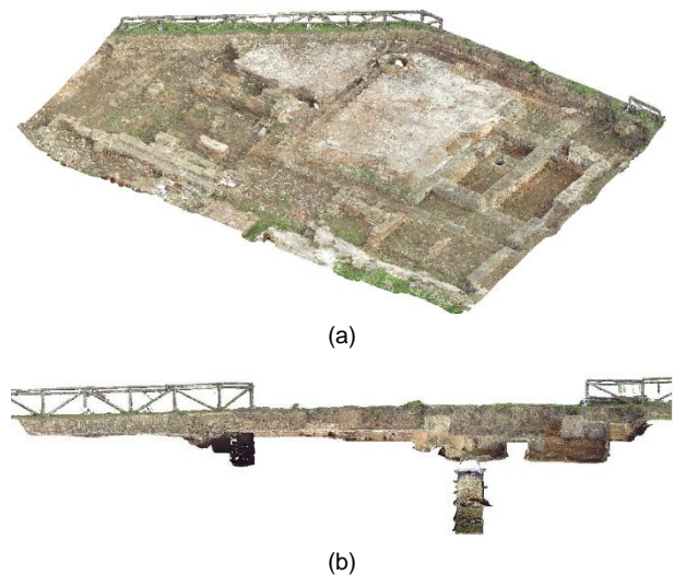
Figure 10: Sanctuary of Isis: a) final point cloud of 70 million points from TLS survey; b) point cloud section with the underground structures.
