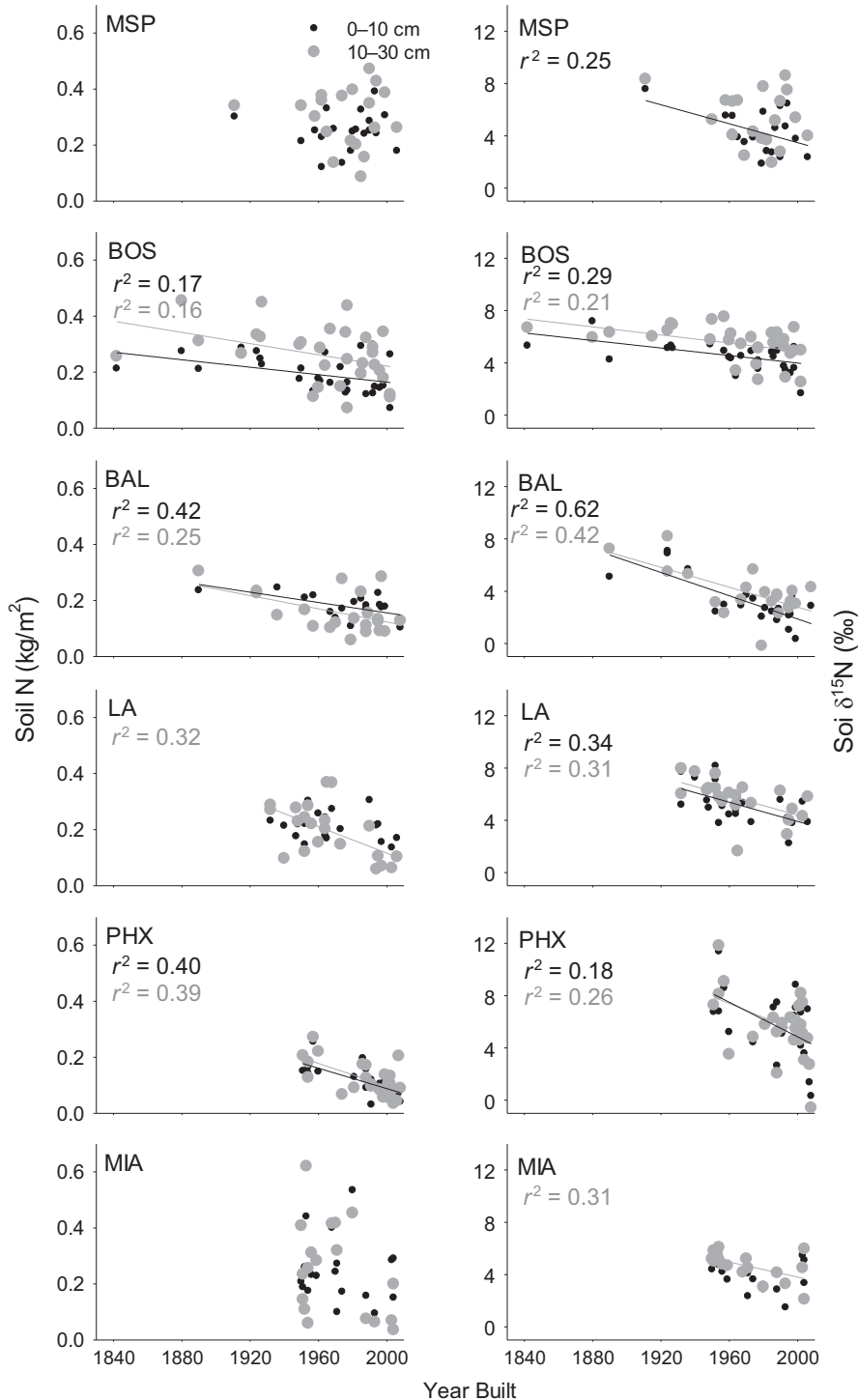
FIG. 7. Relationship between soil N (kg/m 2 ) and soil δ 15 N (‰) with the year the residence was built for the surface soil (black, 0–10 cm) and the subsoil (gray, 10–30 cm) in MSP, BOS, BAL, LA, PHX, and MIA.
