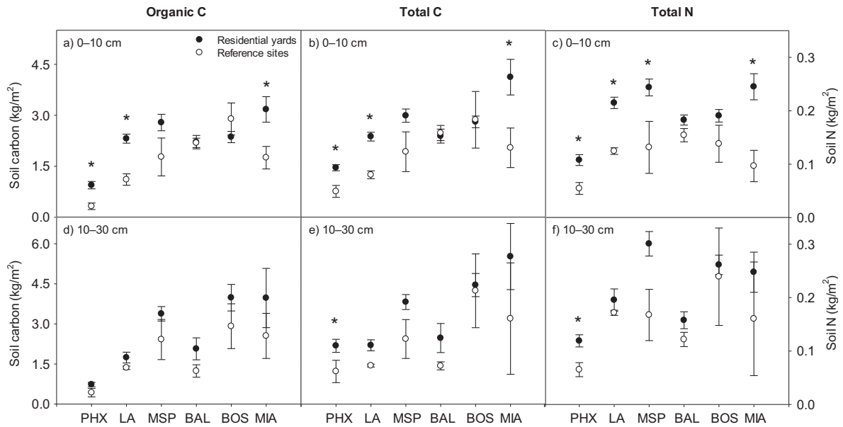
FIG. 2. Mean soil organic C, total C, and total N (kg/m 2 ) in the surface (0–10 cm) and subsurface (10–30 cm) soil layers are shown for residential yards (black) and reference sites (white). Cities are shown in order of increasing mean annual precipitation (MAP), from driest (Phoenix, Arizona; PHX) to wettest (Miami, Florida; MIA). Asterisks represent significant differences ( P \leq 0.05 ) in soil C or N between residential yards and reference sites. Error bars show \pm 1 SE. BOS, Boston, Massachusetts; BAL, Baltimore, Maryland; LA, Los Angeles, California; MSP, Minneapolis-St. Paul, Minnesota.
