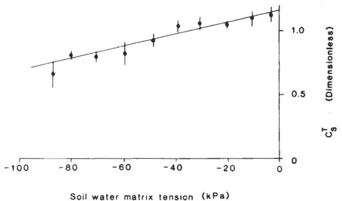
Figure 5 — Mean value and standard error of the function C S T for values of the average soil water matrix potential to a depth of 1 m expressed in kPa. Also shown is the line of linear regression described in the text.
