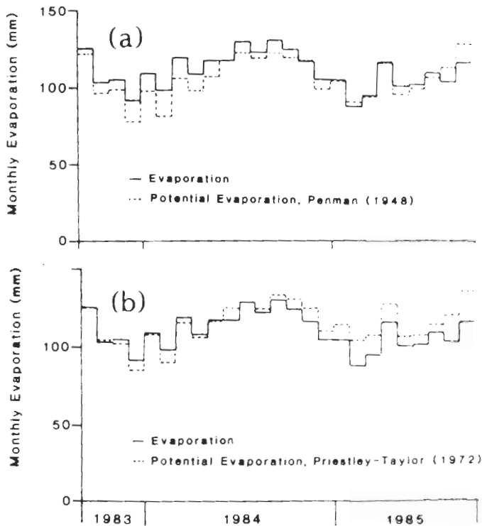
Figure 9 — (a) Monthly values of evaporation, E , and estimates of potential evaporation made with the Penman equation, E_p (see text), in mm for the 25 month experimental period. (b) Monthly values of evaporation and estimates of potential evaporation made with the Priestley-Taylor equation, E_{pT} (see text), in mm for the 25 month experimental period.
