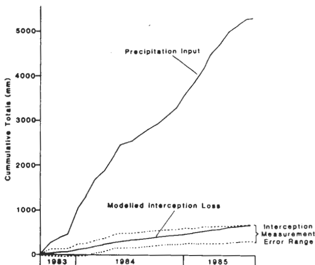
Figure 2 — Cumulative values for precipitation and model calculated interception loss for the experimental period over which interception measurements were made. Also shown is the range within which cumulative interception lies within one standard error of the experimentally measured interception loss.
