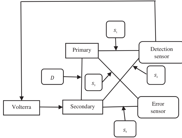
Figure 1. Schematic diagram of geometrical layout of single channel feedforward ANC system. 28
