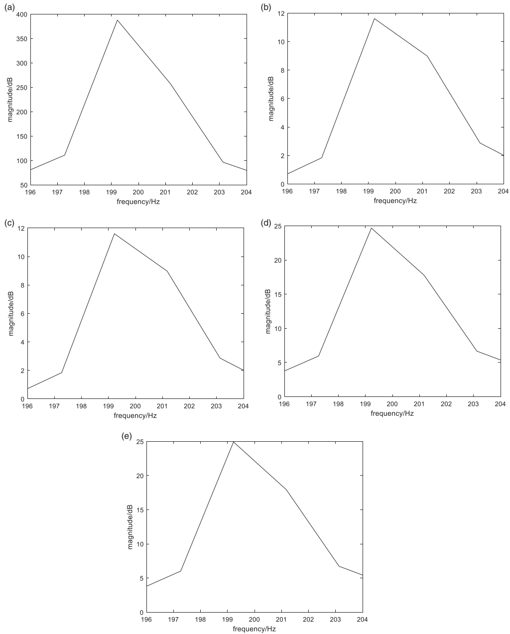
Figure 3. Cancellation performance of narrowband noise in frequency domain: (a) original noise, (b) first distance ratio, (c) second distance ratio, (d) third distance ratio and (e) fourth distance ratio.
