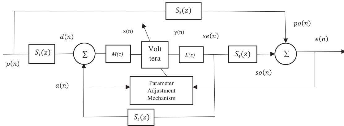
Figure 2. Block diagram of single-channel feedforward ANC system.
