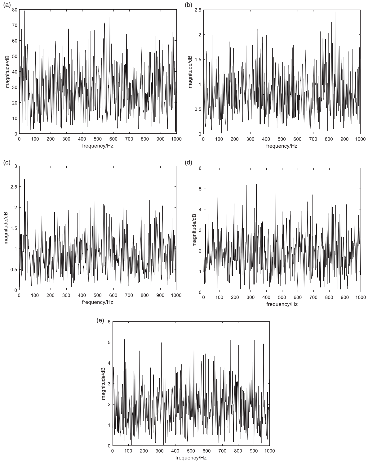
Figure 4. Cancellation performance for broadband noise: (a) original noise, (b) first distance ratio, (c) second distance ratio, (d) third distance ratio and (e) fourth distance ratio.
