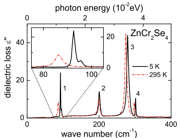
Fig. 2. (Color online) Dielectric loss vs. wave number of \text{ZnCr}_2\text{Se}_4 for 5 K (solid line) and 295 K (dash-dotted line). The inset shows an enlarged region around 90 \text{ cm}^{-1} to document the phonon splitting at low temperatures.
