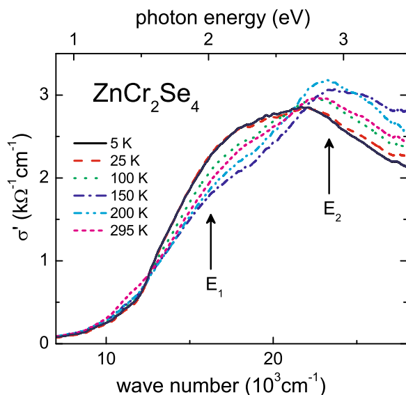
Fig. 4. (Color online) Real part of the conductivity vs. wave number of \text{ZnCr}_2\text{Se}_4 between 0.9 and 3.5 eV for a series of temperatures. The temperatures are given in the figure, the arrows roughly indicate the energies of the electronic transitions.
