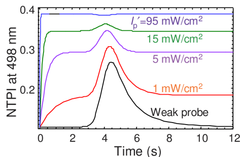
Fig. 7. Variation of NTPI at 498 nm for input pulse at 390 nm with time for different I_p' values in F86D/L40T-ppR, with \Delta t = 1 \text{ s} , I_{m0}' = 50 \text{ mW/cm}^2 for C = 47.02 \mu\text{M} .
