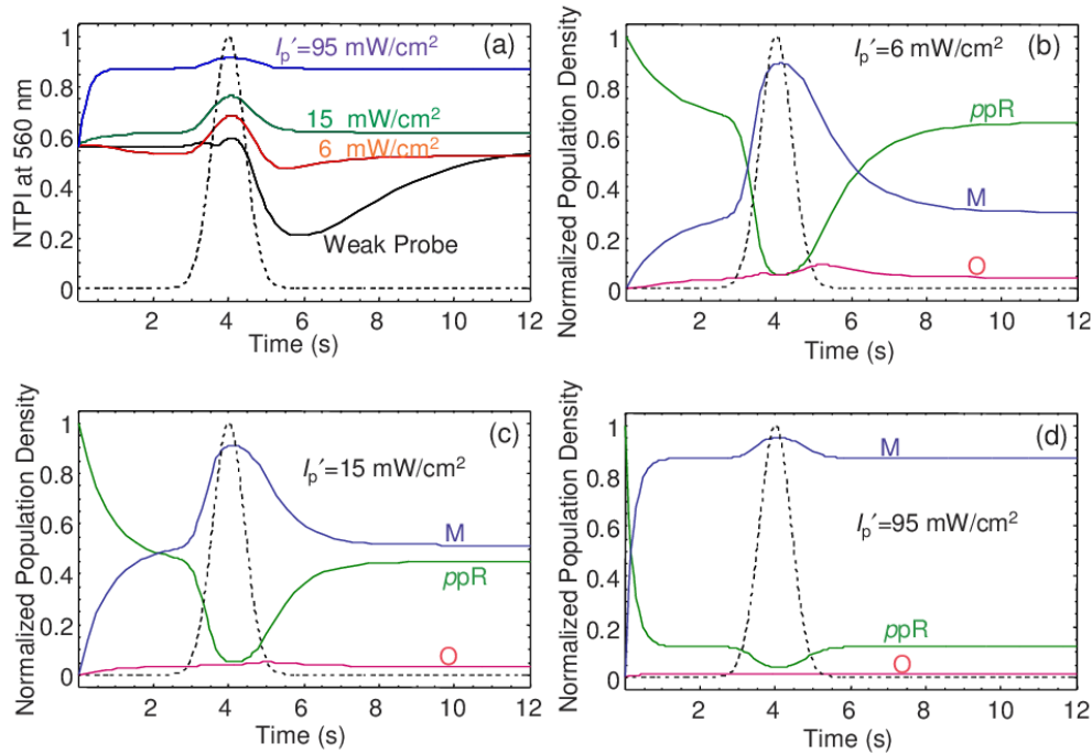
Fig. 4. (a) Variation of NTPI at 560 nm for normalized input pulse at 498 nm (dashed line) with time for different I_p' values in WT- ppR , and variation of the normalized population density of ppR , M and O states for normalized input pulse at 498 nm (dashed line) with time for (b) I_p' = 6 mW/cm 2 , (c) I_p' = 15 mW/cm 2 and (d) I_p' = 95 mW/cm 2 , for \Delta t = 1 s, I_{m0}' = 50 mW/cm 2 , C = 120 \mu M.
