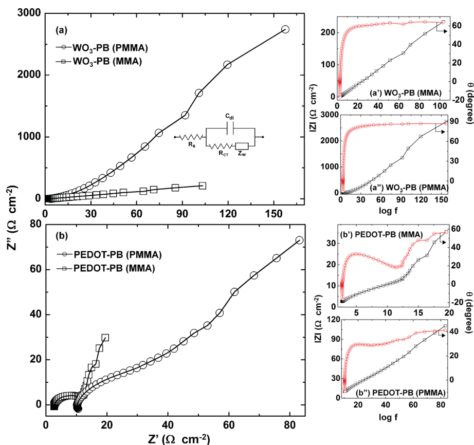
Fig. 9 Nyquist plots of (a) \text{WO}_3\text{-PB(MMA)} ( \square ) and \text{WO}_3\text{-PB(PMMA)} ( \circ ) devices recorded under an ac amplitude of 10 mV; (a', a'', b' and b'') are the corresponding Bode plots ( \square ) |Z| versus \log (frequency) and ( \circ ) \theta versus \log (frequency). The symbols represent the experimental data and the solid lines (—) are obtained by fitting the experimental data in the model shown in (a).
