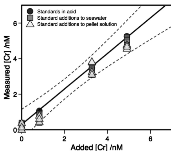
Fig. 1. The results of Cr standard additions to seawater (squares) and to pellet solutions (triangles) are plotted against an external calibration of Cr standards in 1% \text{HNO}_3 (circles). The solid black line shows the slope of the external calibration, with a 99% confidence belt shown as a dashed line. The slopes are as follows: Standards in acid = 1.00, standard additions to seawater = 1.00, and standard additions to pellet solutions = 0.98.
