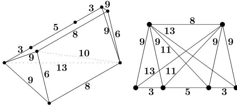
Figure 3. 3-dimensional integral point set consisting of 8 points with minimum diameter.
