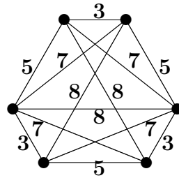
Figure 4. Smallest integral hexagon.
