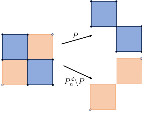
FIG. 9. An example of a failure of symmetry for the cubical complex. The dark squares indicate open sites. The complement of the open sites is different (bottom right) than the union closed sites. In particular, the latter is connected (via the point in the middle), while the former is not.
