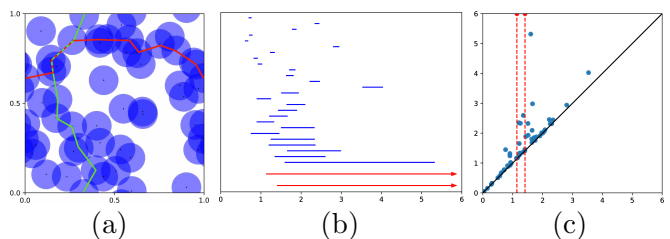
FIG. 1. Persistent homology for a point sample on the 2D flat torus (a unit box with periodic boundary conditions). (a) A set of 50 points \mathcal{X} sampled from the flat torus. The filtration X_t taken here is the union of balls of radius t around the points. We increase t from 0 to \infty and calculate \text{PH}_1 . (b) The barcode for \text{PH}_1 . Each 1-cycle is represented by a bar, where the endpoints are the radii in which the cycle was formed and filled in (birth, death). The two red bars correspond to the two cycles in the torus (“the giant cycles”) while the blue ones are considered as “noise”. (c) The persistence diagram for \text{PH}_1 . Here the (birth, death) pairs are plotted as points in the plane. Two points are far away from the diagonal (shown by the red dashed line), representing the true non-trivial or giant cycles of the torus. This figure was generated using the GUDHI package [10].
