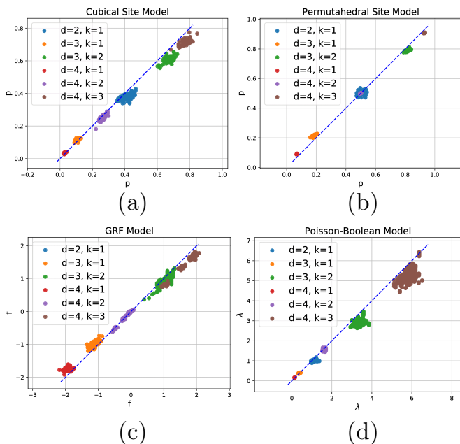
FIG. 8. Appearance of giant cycles vs. emerging of the Betti numbers. The x-coordinate of each point corresponds to the appearance time of the k -th giant cycle, while the y-axis is the time at which the equality \beta_i = \beta_{i-1} occurs. The plots provide strong experimental evidence that the appearance of higher dimensional cycles occurs in the vicinity of this equality. (a) Cubical site model (b) Permutahedral site model (c) Gaussian random field (d) Poisson-Boolean.
