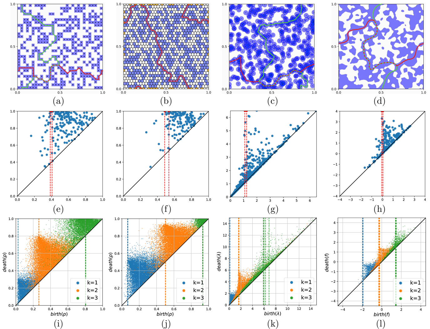
FIG. 3. The emergence of the giant 1-cycles in 2D for (a) the cubical site model Q(n, p) with (n = 2500, p = 0.43) , (b) the permutahedral site model P(n, p) with (n = 1024, p = \frac{1}{2}) , (c) Poisson-Boolean model B(n, \lambda) with (n = 500) , and (d) the GRF model G(\alpha) (computed on a 512 \times 512 grid). The red and green lines mark the two giant 1-cycles (recall the period boundary gluing). Note in P(n, p) that only one giant cycle has appeared and that it is the sum of the two “obvious” giant cycles. (d-g) \text{PH}_1 for the corresponding models with the red vertical lines mark the birth times of the giant 1-cycles. (h-l) The persistence diagrams for the corresponding models for d = 4 . In this case we have homology in degrees k = 1, 2, 3 . The vertical lines mark the birPth times of the giant k -cycles. The relevant scale parameter is n = 65536 for Q(n, p) , P(n, p) , as well as the grid size for the GRF model. For B(n, \lambda) , n = 5000 .
