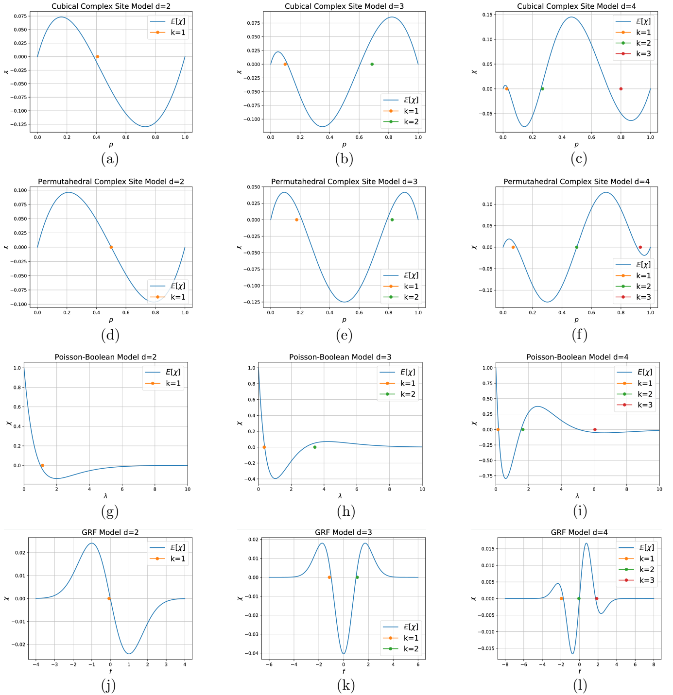
FIG. 4. The expected EC curve and the giant cycles. In each plot we draw the expected EC curve (solid line), along with the birth time of the first giant k -cycle for k = 1, \dots, d-1 (dots). (a)-(c) The random cubical complex. (d)-(f) The random permutahedral complex. (g)-(i) The Boolean model. (j)-(l) The Gaussian random field. We simulated all the models on the d -dimensional torus, for d = 2, 3, 4 (from left to right).
