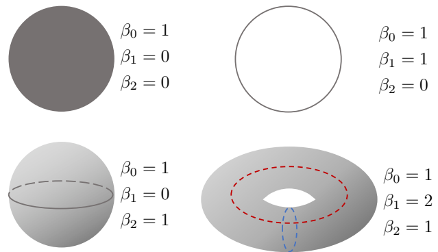
FIG. 2. Example of simple topological spaces with their Betti numbers. From left to right - a disc, a circle, a 2-dimensional sphere, and a 2-dimensional torus. For the torus, we marked the two 1-cycles in dashed lines.
