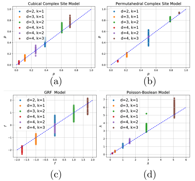
FIG. 6. Appearance of giant cycles vs. zeros of the expected EC curve. The x-coordinate of each point is the corresponding zero of the expected EC curve, and the y-coordinate is the value when a giant k -cycle appears, (a) Cubical site model (b) Permutahedral site model (c) Gaussian random field (d) Poisson-Boolean.
