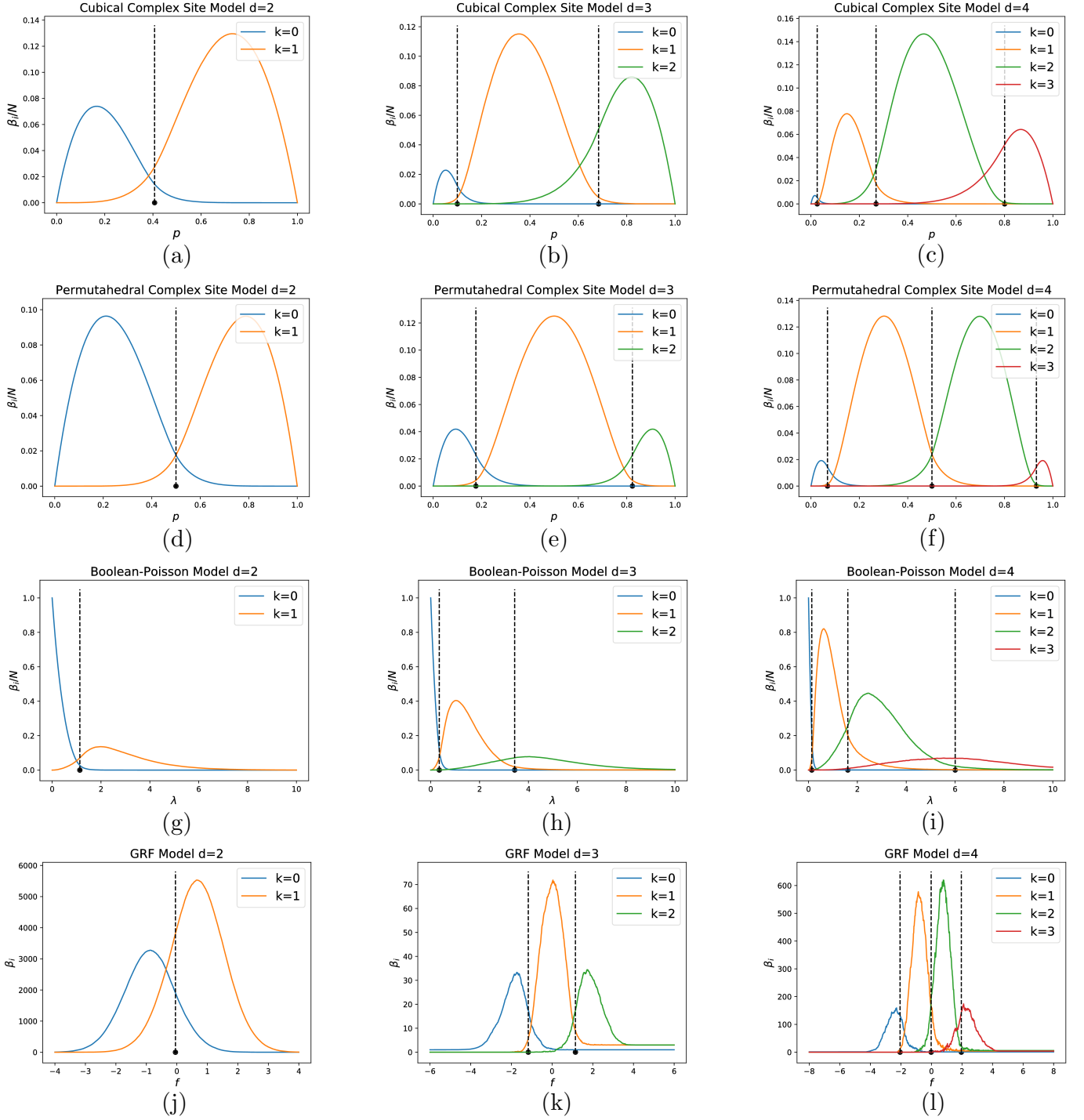
FIG. 7. The empirical (average) Betti curves and the giant cycles. In each plot, we draw the Betti curves (solid line), along with the birth time of the first giant k -cycle for k = 1, \dots, d - 1 . (a)-(c) The random cubical complex. (d)-(f) The random permutahedral complex. (g)-(i) The Boolean model. (j)-(l) The Gaussian random field. We simulated all the models on the d -dimensional torus, for d = 2, 3, 4 (from left to right).
