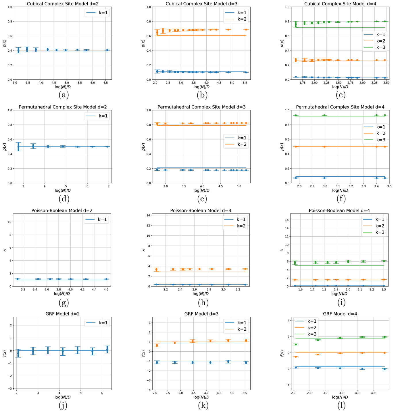
FIG. 5. Statistics for the birth time of the giant k -cycles. For each model we repeated the simulations in order to estimate the mean and variance of the birth time of the first giant k -cycle. In each figure the x-axis is \log n , and the y-axis represent the parameter value ( p , \lambda , or \alpha ). The dots represent the mean value estimate, and the bars around them follows the standard deviation. The horizontal lines mark the corresponding zeros of the EC curve. (a)-(c) The random cubical complex. (d)-(f) The random permutahedral complex. (g)-(i) The Boolean model. (j)-(l) The Gaussian random field.
