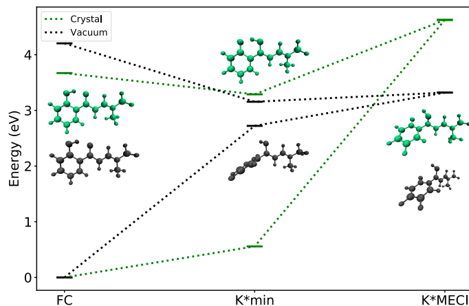
Fig. 8 Calculated energies and geometries at critical points on PES. Crystal geometries obtained with ONIOM((TD)- \omega B97X-D/6-31G(d):AMBER), with energies calculated at MS-3-CASPT2(12,11):AMBER. Vacuum geometries obtained with (TD)- \omega B97X-D/6-311++G(d,p) and energies obtained with MS-3-CASPT2(12,11). The average energy of the S_1 and S_0 states is shown for the MECI.
