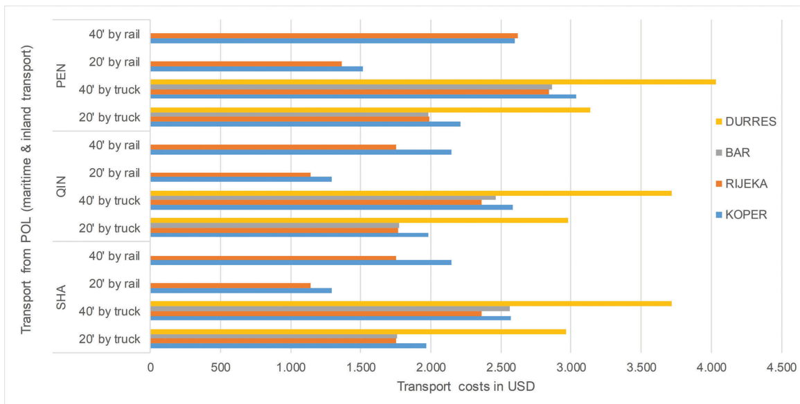
Figure 5 Comparison of transport costs from POL to the final destination in Belgrade Slika 5. Usporedba troškova transporta iz luka ukraja do krajnjega odredišta u Beogradu
