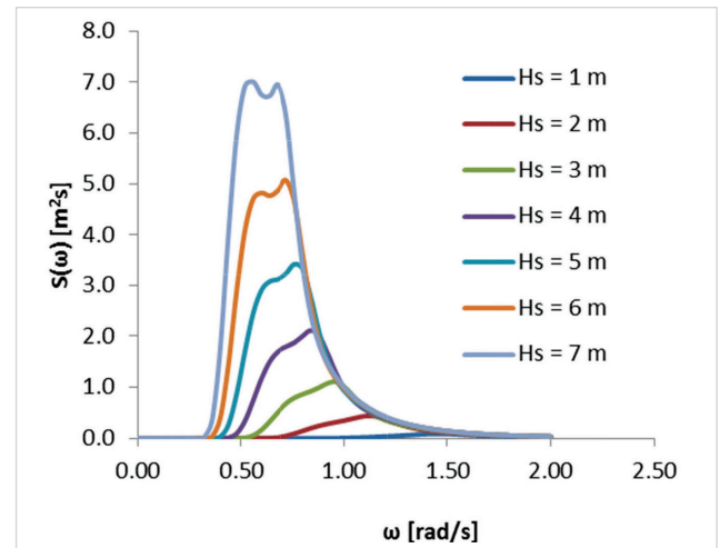
Figure 4 Failure of Tabain's wave spectrum in combination with the optimized modal frequency model
