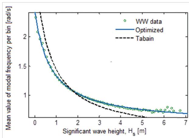
Figure 3 Parameter optimization of Tabain's modal frequency relation
