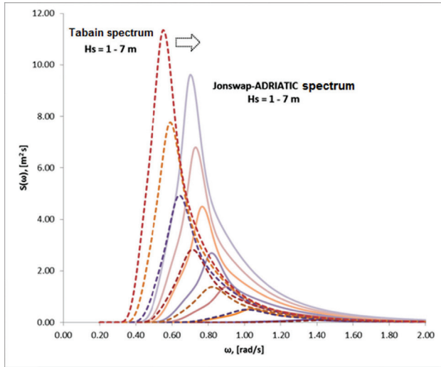
Figure 5 Transformation of Tabain's wave spectrum into the JONSWAP-Adriatic wave spectrum
