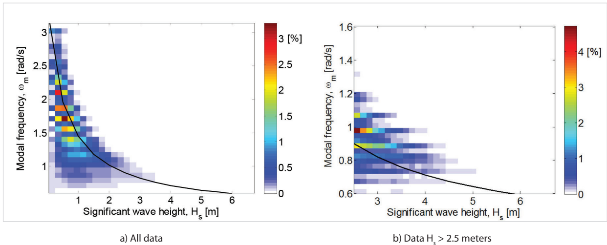
Figure 2 Frequency of occurrence distribution of significant wave height and modal frequency. WW scattered data compared with Tabain's formulation (black line)
