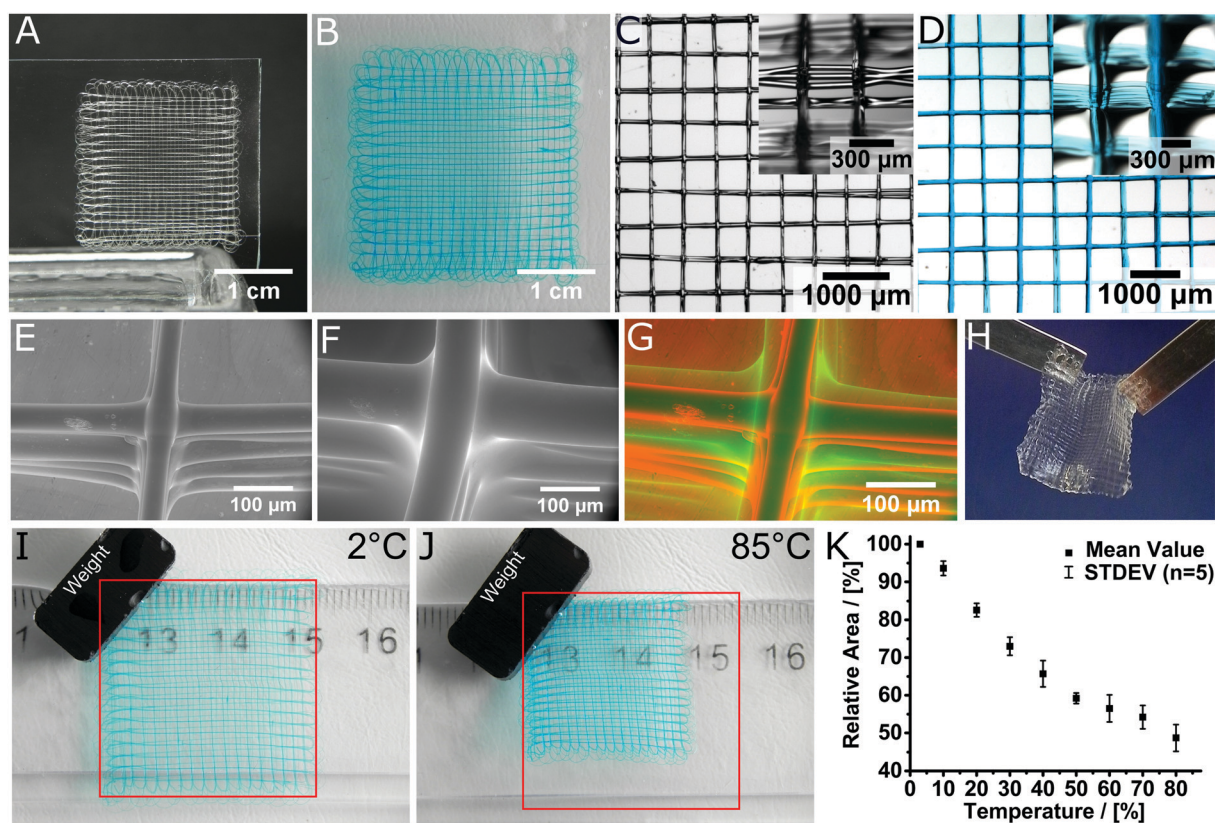
Fig. 3 Layered structure of the MEW printed scaffold in the (A) dry state and (B) swollen state. Stereoscopic image of (C) the dry and (D) swollen scaffold, hydrated and stained with DY-647P1-maleimide for improved visualization. Insets show the scaffolds from a tilted angle to better visualize the fibre morphology and stacking. ESEM image of (E) the dried and (F) swollen structure. (G) Visualization of the volume decrease by superposition of the dried and swollen 3D hydrogel scaffold. (H) Scaffolds are mechanically robust and can be easily handled and transferred. Temperature dependent swelling of the hydrogel architectures visualized at (I) 2 °C and (J) 85 °C. The red square indicates the size of the scaffold at 2 °C. (K) Relative area of the scaffolds depending on the temperature. Video 1 (ESI†) shows the hydration process while Video 2 (ESI†) shows the thermoresponsiveness of the samples shown in (I and J).
