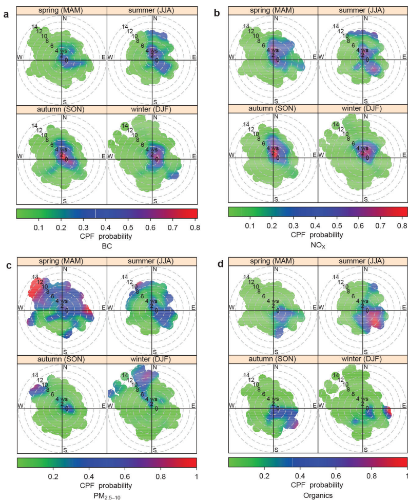
Fig. A8. Bivariate polar plots for (a) BC, (b) NO x , (c) PM 2.5-10 and (d) organics showing the highest pollutant concentration (75th percentile) for different wind speed and direction bins.
