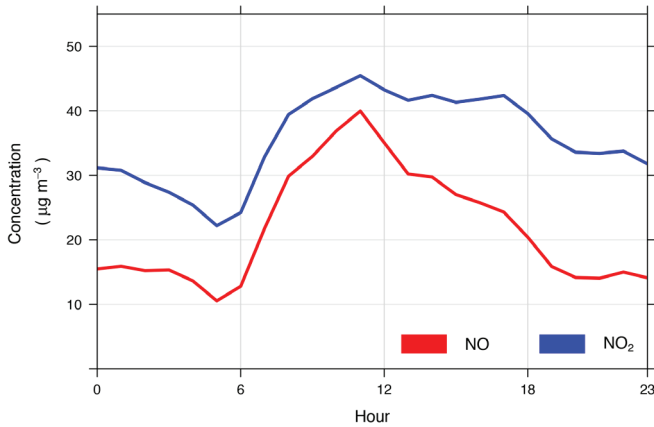
Fig. A9. Diurnal variations of NO and NO 2 during different seasons in the Helsinki city centre.
