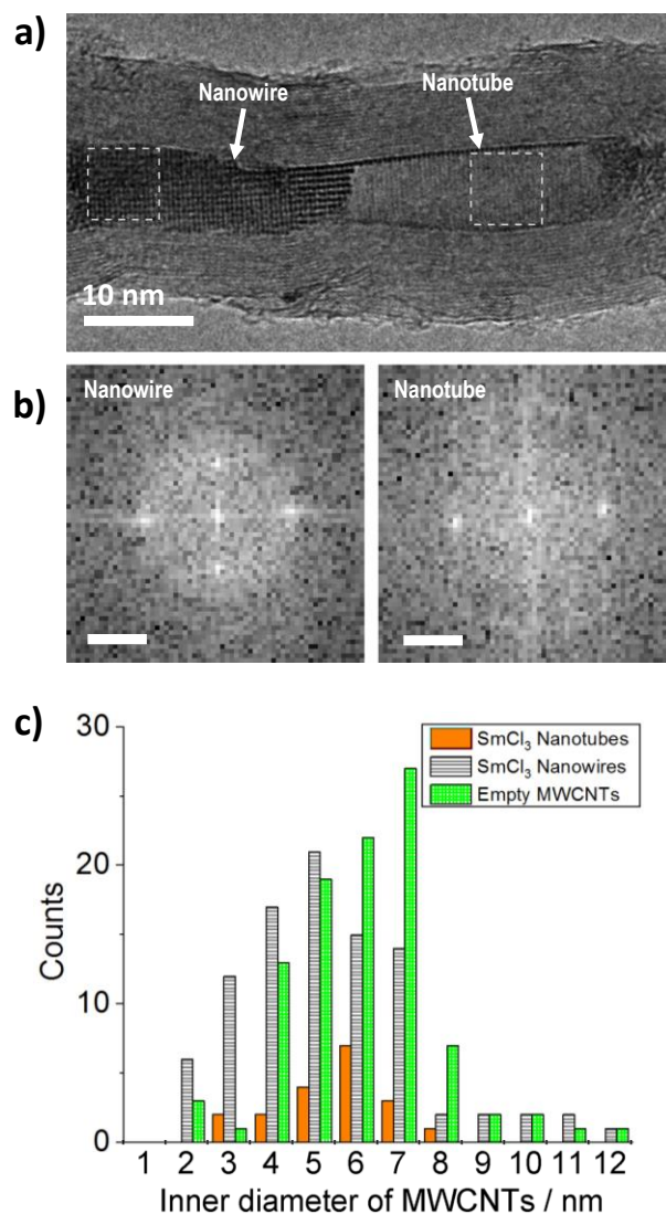
Figure 4. a) HRTEM image of SmCl 3 @MWCNTs filled at 1200 °C revealing the presence of both SmCl 3 nanotubes and nanowires inside the cavities of the MWCNTs. b) FFT of the areas marked with squares in a) showing the crystalline nature of both nanowires and nanotubes (scale bar = 2 nm -1 ). c) HRTEM images statistical analysis of the amount of SmCl 3 inorganic nanotubes and nanowires present in the sample.
