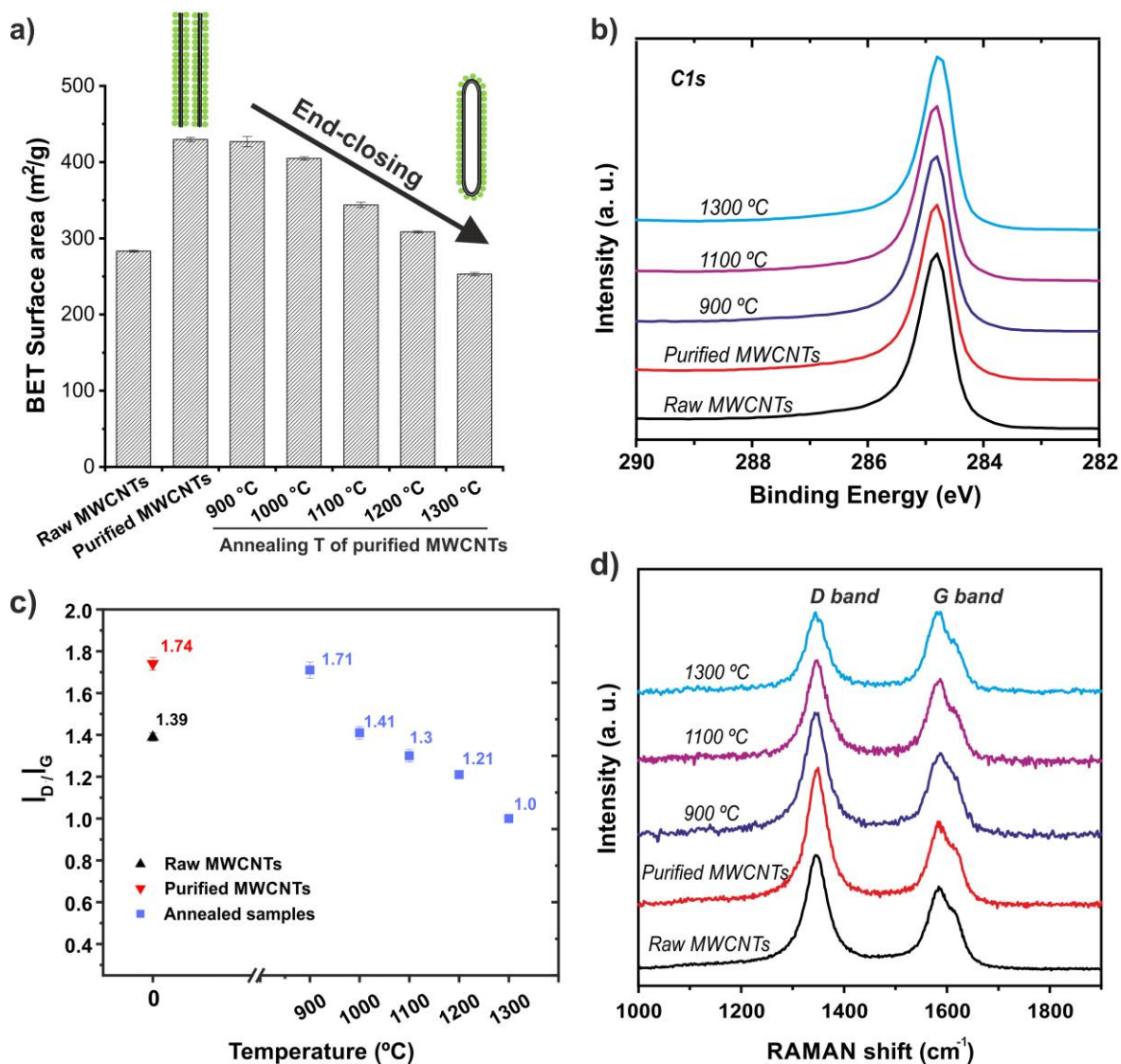
Figure 1. a) BET surface area (Schematic representation: black lines – MWCNTs; green dots – N 2 molecules), b) normalized XPS spectra over the C1s region, with the C1s peak set to a BE of 284.8 eV, c) I D /I G Raman ratios and d) normalized Raman spectra of raw, purified MWCNTs (2 h steam and HCl), and purified MWCNTs after being annealed at different temperatures (between 900 - 1300 °C).
