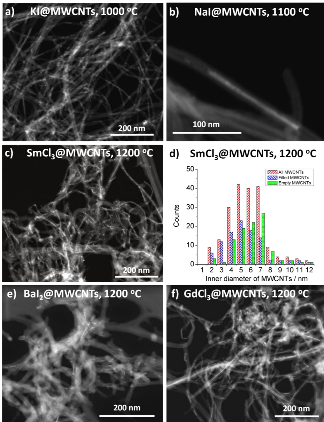
Figure 2. Multi-walled carbon nanocapsules of a) KI@MWCNTs prepared at 1000 °C, b) NaI@MWCNTs at 1100 °C, c) SmCl 3 @MWCNTs at 1200 °C, d) histogram showing the inner diameter distribution and the amount of empty, filled and both filled and empty (all) MWCNTs in a sample of SmCl 3 @MWCNTs prepared at 1200 °C, e) BaI 2 @MWCNTs at 1200 °C and f) GdCl 3 @MWCNTs at 1200 °C.
