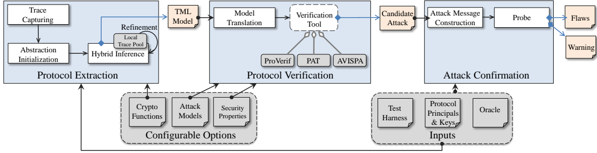
Figure 2: Overview of AUTHSCAN
