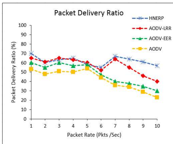
Figure 6: HNERP Performance Comparison for Packet Delivery Ratio
