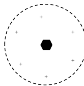
Fig. 1 Stereographic Projection for the Point Group C_6
