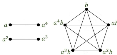
Figure 1: The Conjugate Graph of D_{10} , K_2 \cup K_2 \cup K_5
