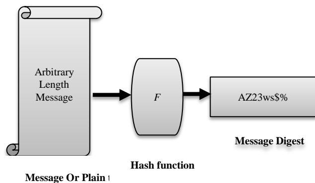
Fig. 1. Hash function.
