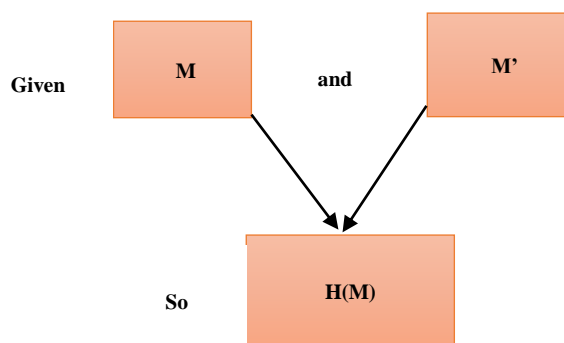
Fig. 2. Collision resistance.
