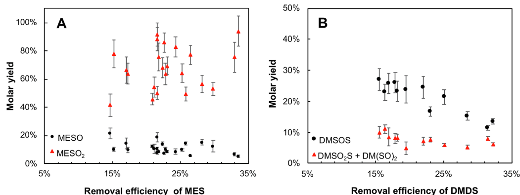
Fig. 7. A) Molar yield of the MESO and MESO 2 as function of removal efficiency of MES. B) Molar yield of DMSOS and the sum of the isomers DMSO 2 S and DM(SO) 2 as function of removal efficiency of DMDS. Only the experiments with removal efficiency superior to 15% were considered due to the extremely high uncertainty at the low range (< 15%).
