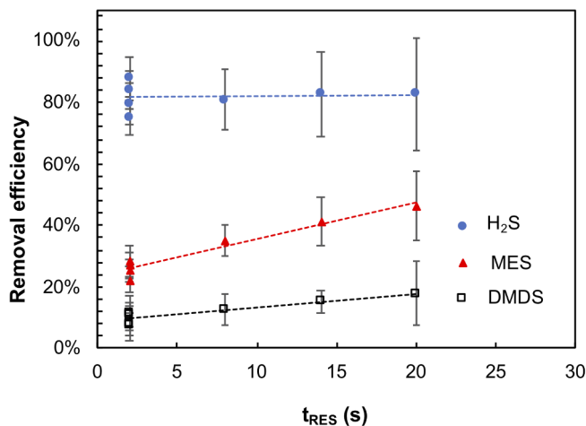
Fig. 2. Removal efficiency of H 2 S, MES and DMDS as function of t RES for [H 2 S] in = 0.46 ± 0.08 ppmv; [MES] in = 1.8 ± 0.2 ppmv; [DMDS] in = 4.0 ± 0.4 ppmv, [O 3 ] in = 100 ppmv and T reactor = 20 °C.
