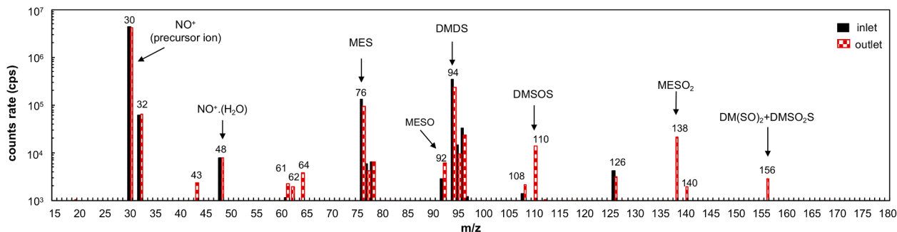
Fig. 6. Comparison of \text{NO}^+ spectra at the reactor inlet with the reactor outlet for [\text{H}_2\text{S}]_{\text{in}} = 0.46 \pm 0.08 ppmv; [\text{MES}]_{\text{in}} = 1.8 \pm 0.2 ppmv; [\text{DMDS}]_{\text{in}} = 4.0 \pm 0.4 ppmv, [\text{O}_3]_{\text{in}} = 100 ppmv, t_{\text{RES}} = 2 s and T_{\text{reactor}} = 60 °C.
