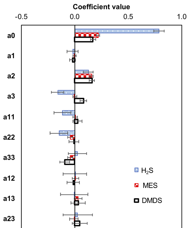
Fig. 4. Coefficient values of Doehlert models for removal efficiencies of H 2 S, MES and DMDS obtained considering a confidential interval of 95%.
