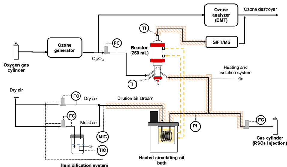
Fig. 1. Experimental set-up.
