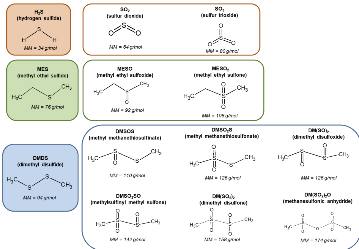
Fig. 5. RSCs and their expected oxidation products according to the reactional mechanism proposed in the literature [24,29,30].
