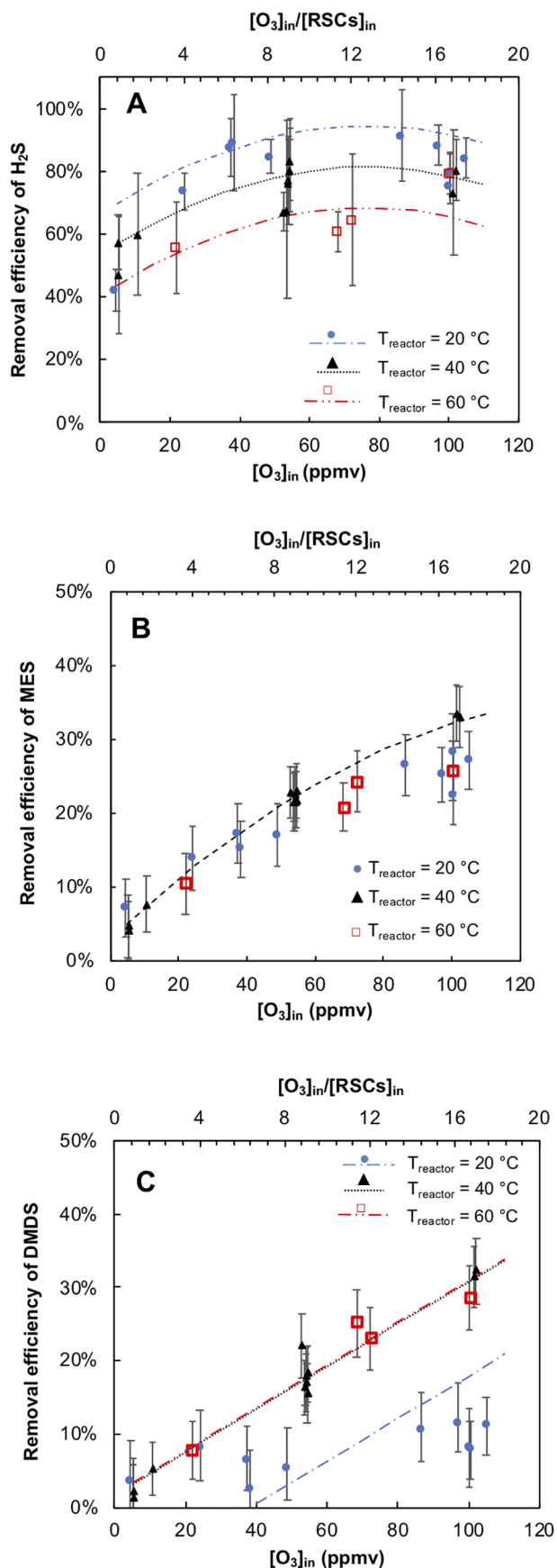
Fig. 3. Removal efficiency of H 2 S (A), MES (B) and DMDS (C) as function of the inlet ozone concentration under different T_{\text{reactor}} , for [\text{H}_2\text{S}]_{\text{in}} = 0.46 \pm 0.08 ppmv; [\text{MES}]_{\text{in}} = 1.8 \pm 0.2 ppmv; [\text{DMDS}]_{\text{in}} = 4.0 \pm 0.4 ppmv and t_{\text{RES}} = 2 s.
