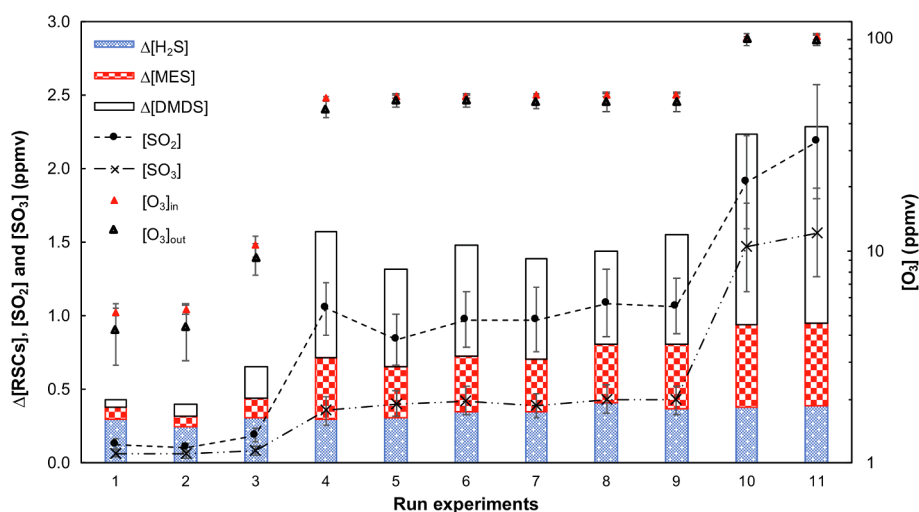
Fig. 8. Comparison of RSCs consumed with the concentration of SO 2 and SO 3 measured at the reactor outlet and with the ozone concentration at the reactor inlet and outlet. Experiments carried out with t_{\text{RES}} of 2 s and T_{\text{reactor}} at 40 °C.
