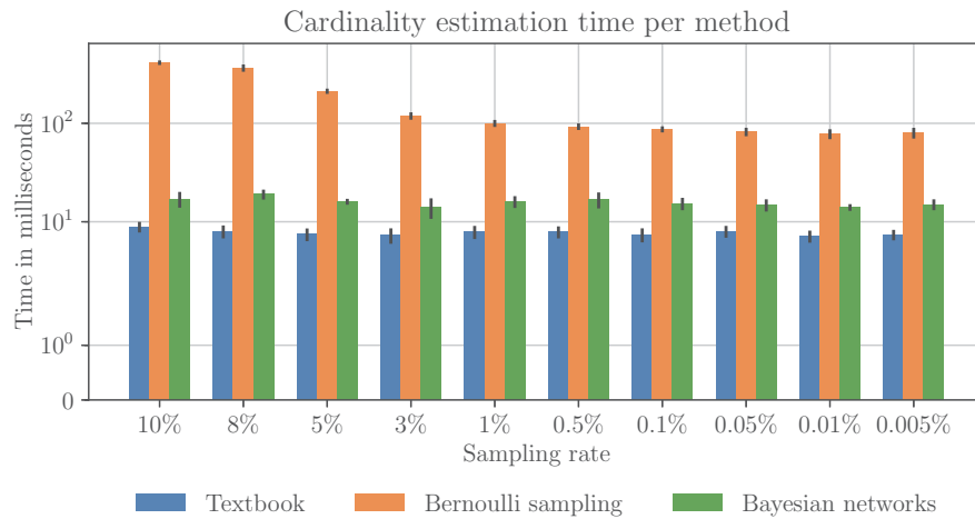
Fig. 5. Cardinality estimation time
