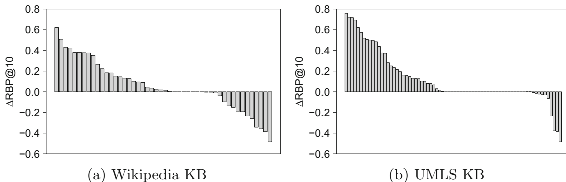
Fig. 3. Changes in RBP@10 between the Entity Query Feature Expansion model utilising the best settings vs. baseline. Only high coverage queries are reported.
