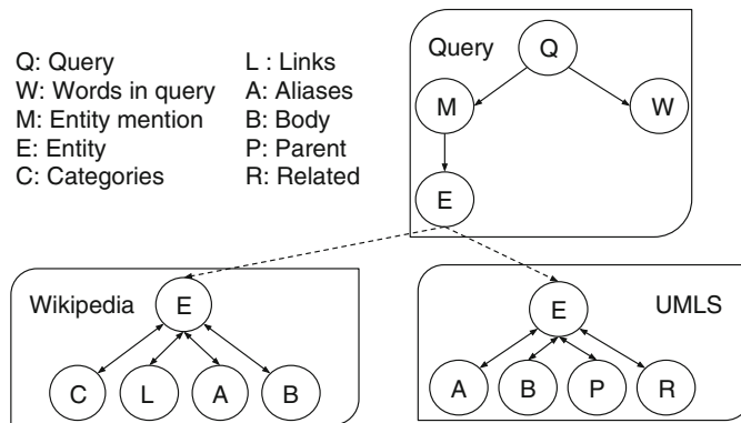
Fig. 1. Summary of expansion sources.
