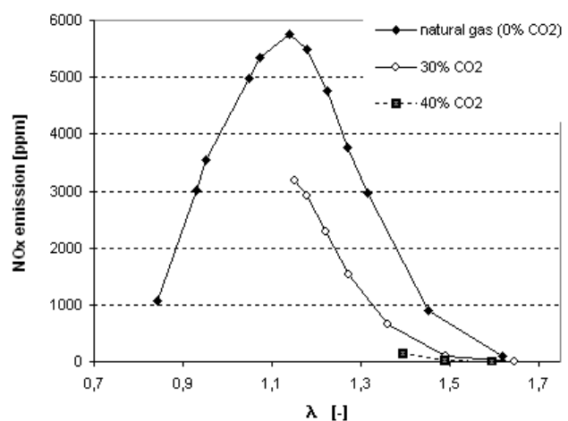
Figure 1. \text{NO}_x emission
