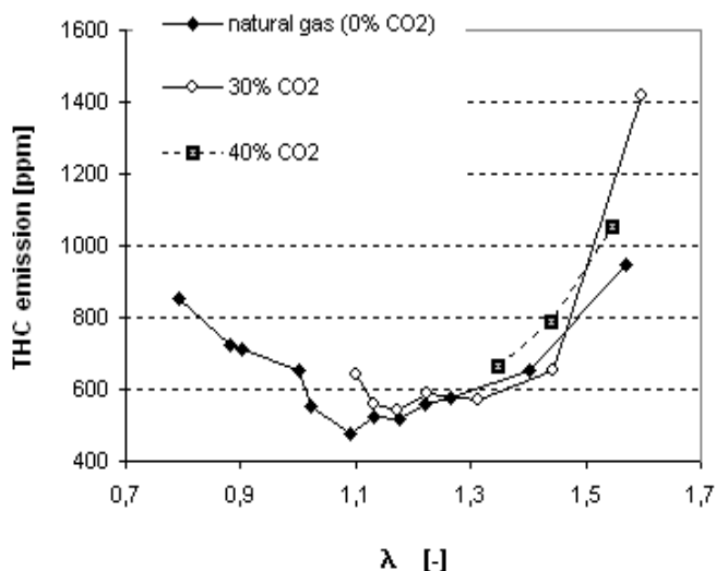
Figure 3. THC emission
